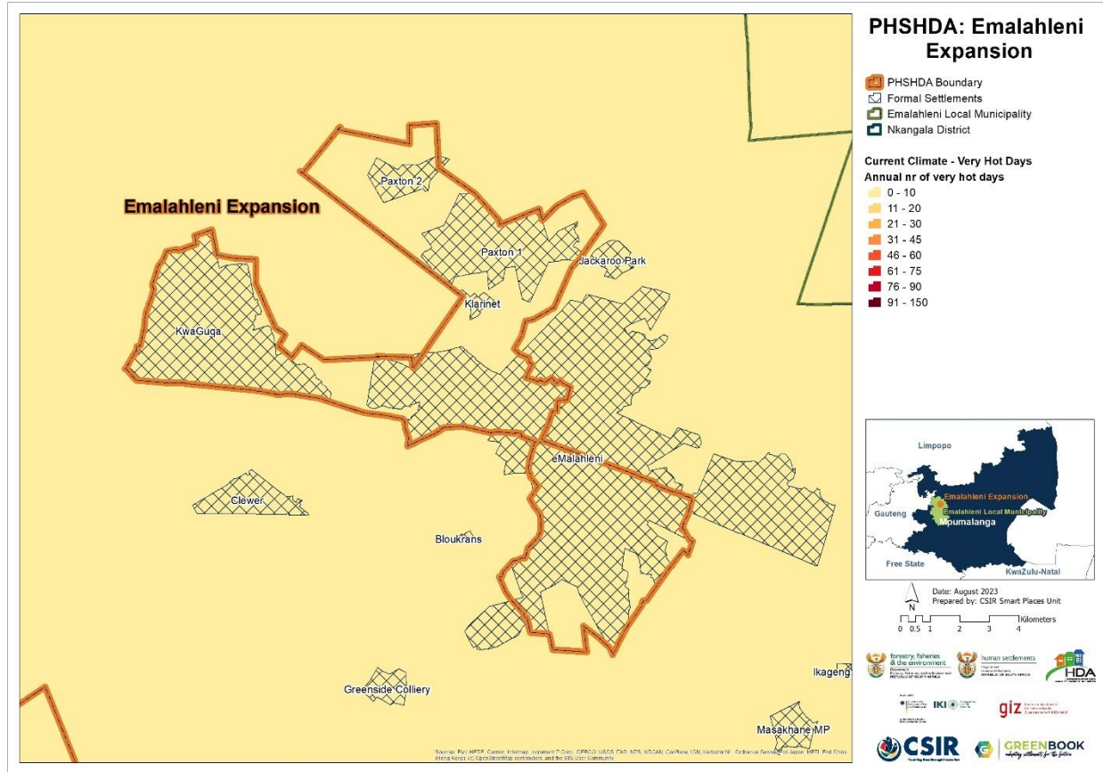
Figure 11: Annual number of very hot days under baseline climatic conditions across Emalahleni Expansion PSHDA with daily temperature maxima exceeding 35 °C
