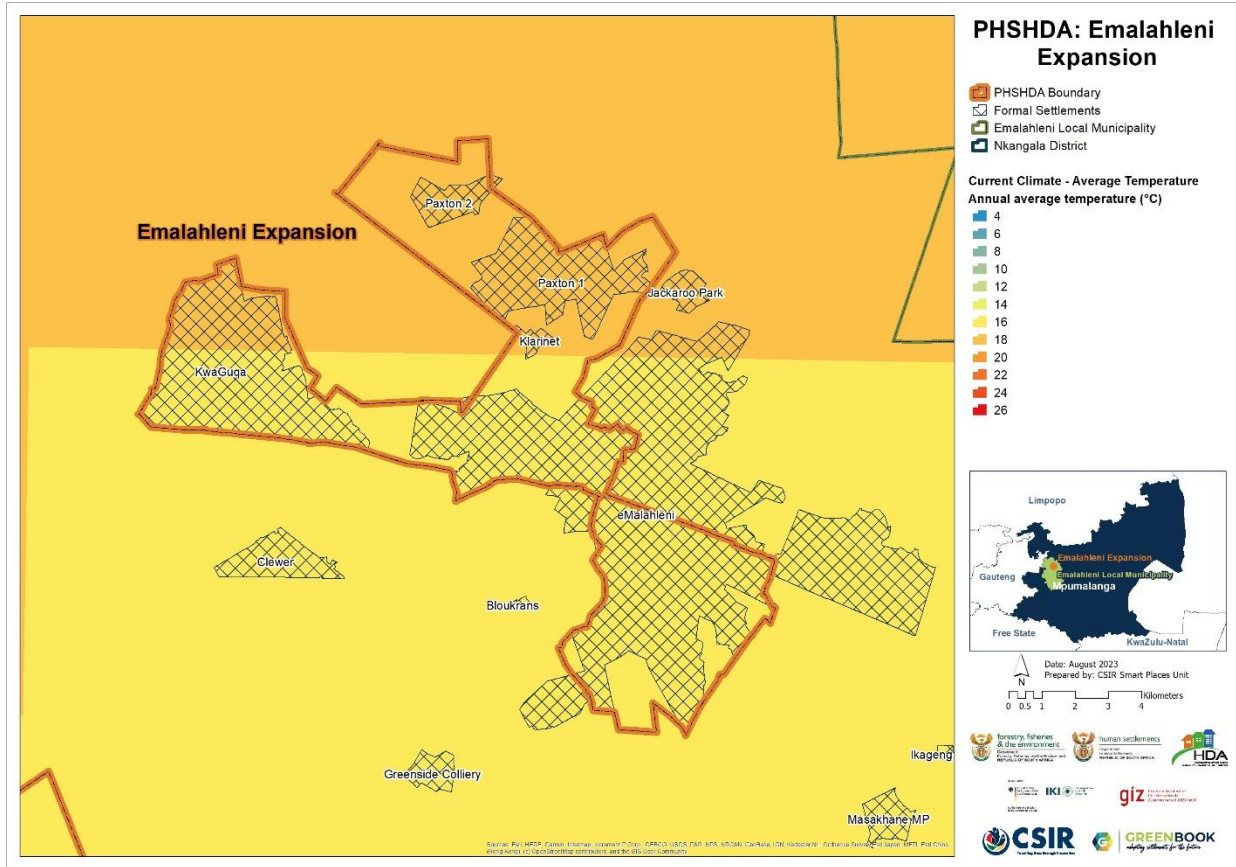
Figure 4: Average annual temperature (°C) for the baseline period 1961 – 1990 for Emalaheni Expansion PSHDA
