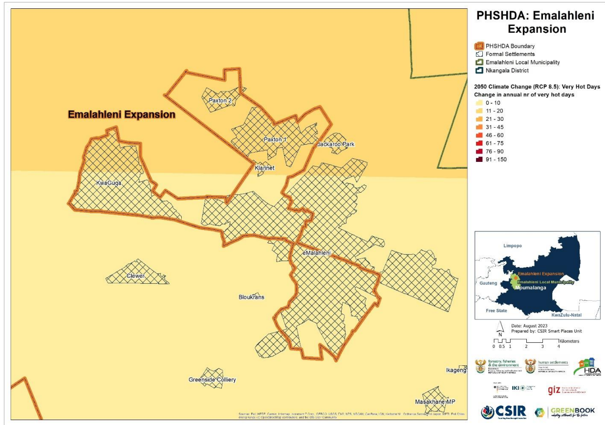
Figure 12: Projected change in annual number of very hot days across Emalahleni Expansion PSHDA with daily temperature maxima exceeding 35 °C, assuming an (RCP 8.5) emissions pathway
