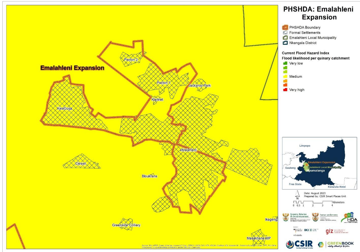
Figure 18: The flood hazard index across Emalahleni Expansion PSHDA under current (baseline) climatic conditions
