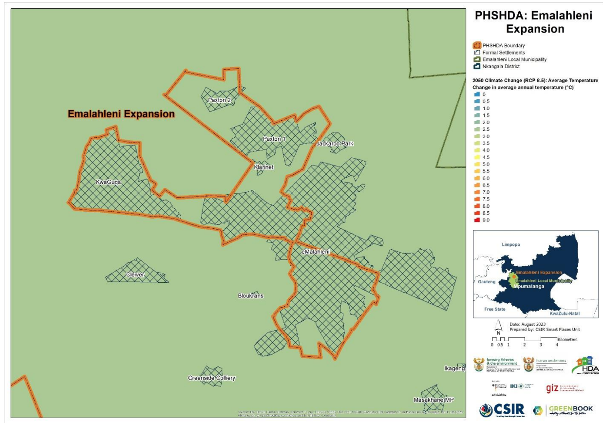
Figure 5: Projected change in average annual temperature (°C) from the baseline period to the period 2021 – 2050 for Emalahleni Expansion PSHDA, assuming an (RCP 8.5) emissions pathway
