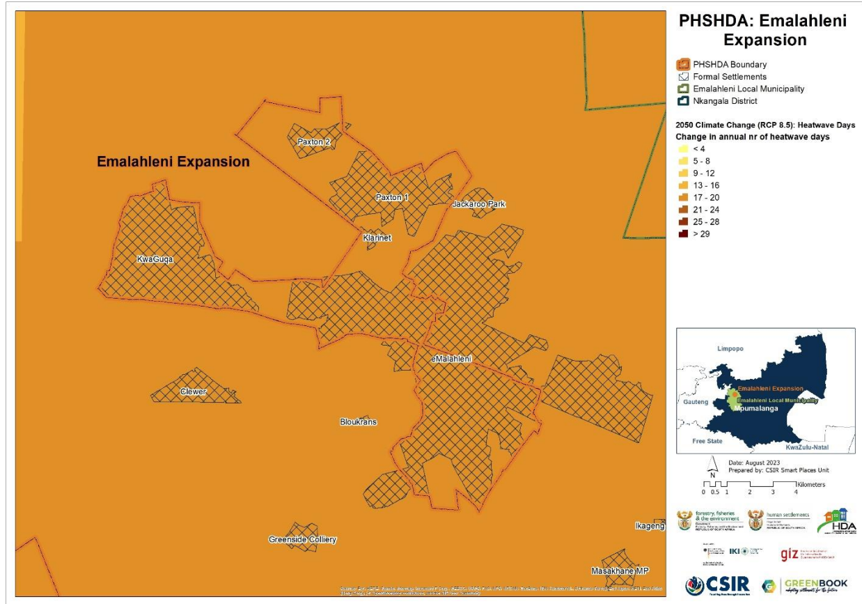
Figure 14: Projected change in annual number of heatwave days across Emalahleni Expansion PSHDA, assuming an (RCP 8.5) emissions pathway
