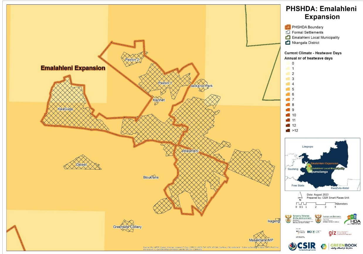
Figure 13: Annual number of heatwave days under baseline climatic conditions across Emalahleni Expansion PSHDA
