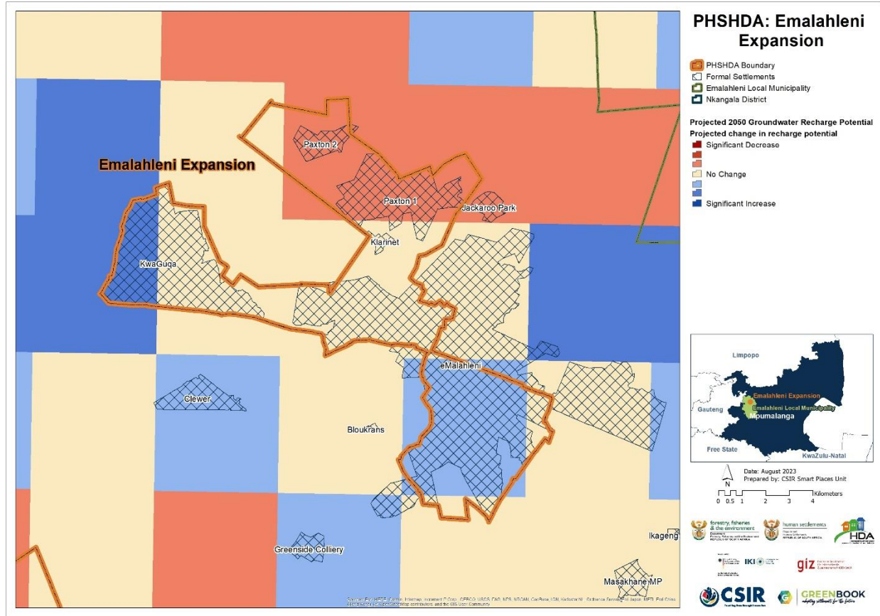
Figure 24: Projected changes in groundwater recharge potential from baseline climatic conditions to the future across Emalahleni Expansion PSHDA
