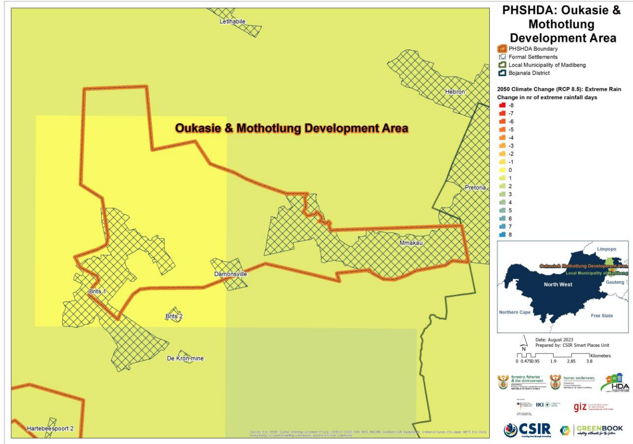
Figure 22: Projected change into the future in extreme rainfall days across OM PSHDA under an RCP 8.5 scenario.
