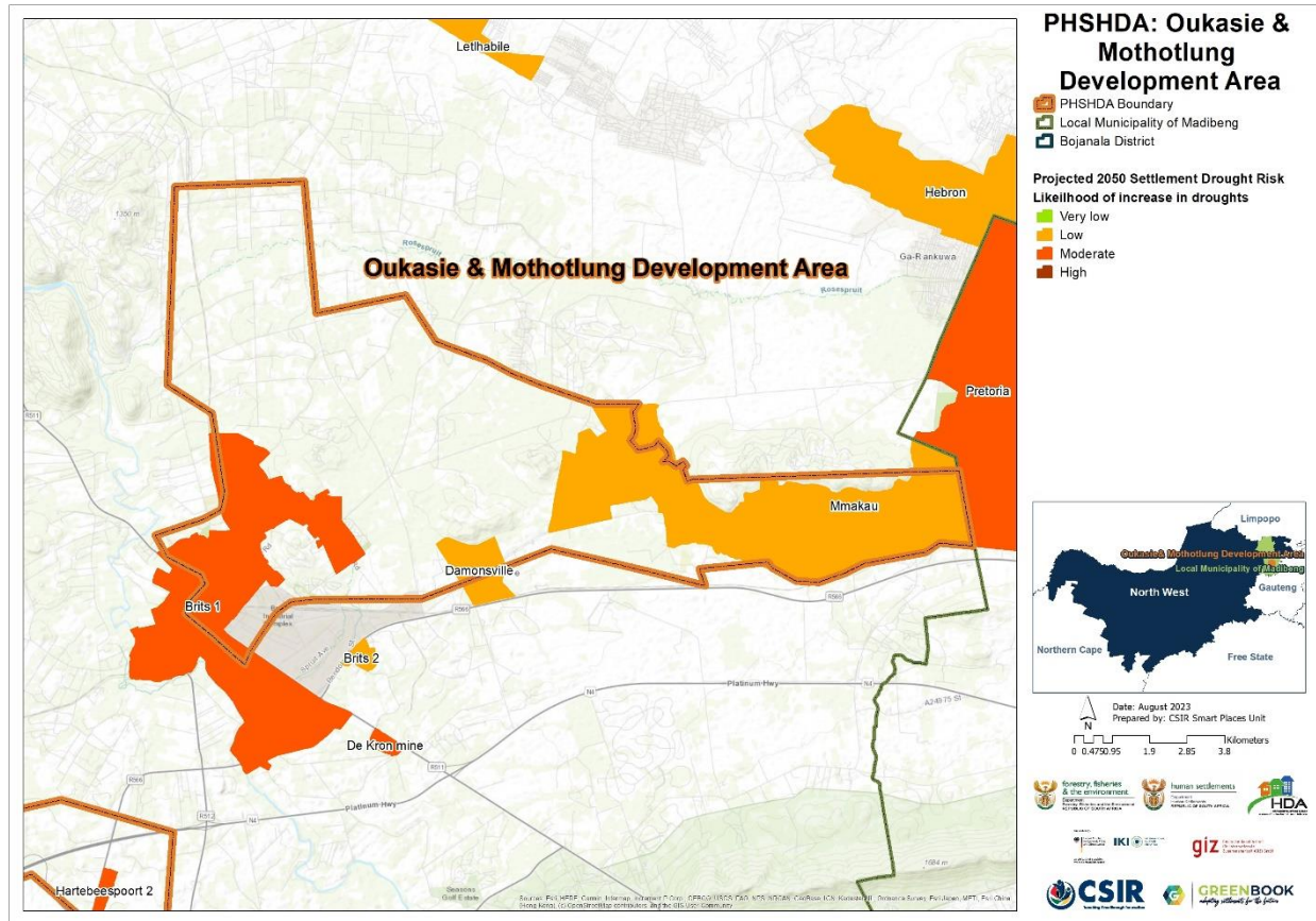
Figure 11: Settlement-level drought risk for OM PSHDA
