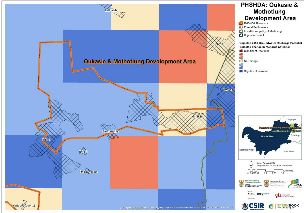
Figure 27: Projected changes in groundwater recharge potential from baseline climatic conditions to the future across OM PSHDA
