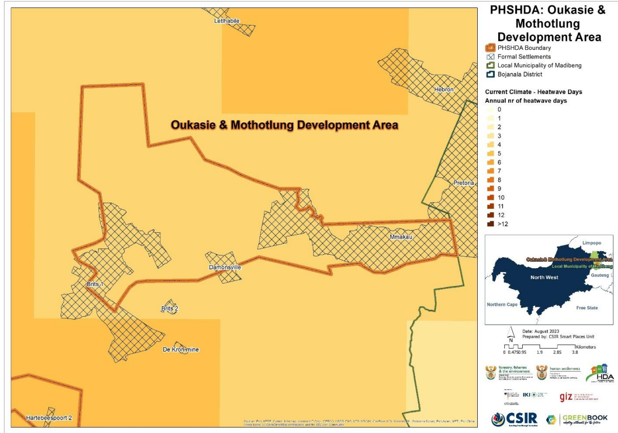
Figure 14: Annual number of heatwave days under baseline climatic conditions across OM PHSFDA
