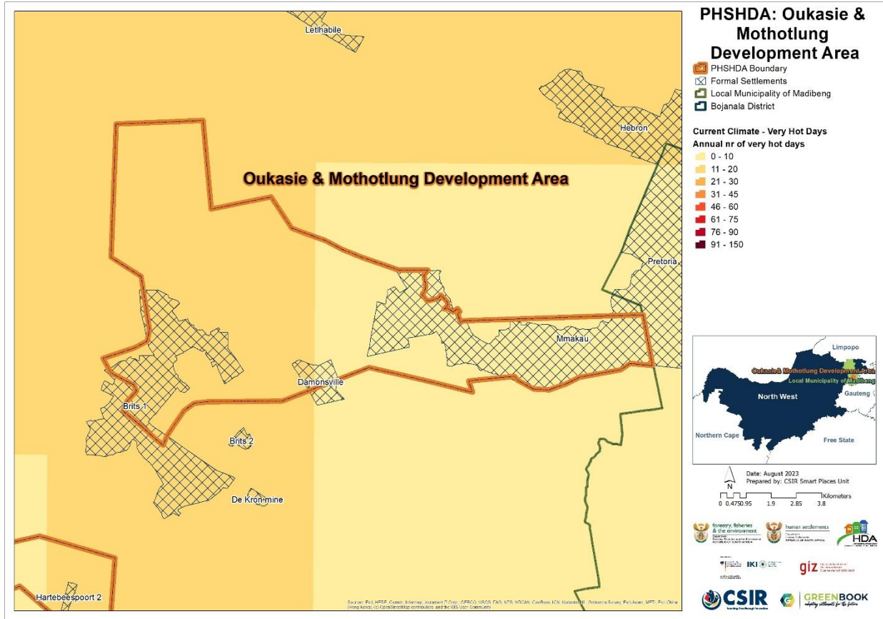
Figure 12: Annual number of very hot days under baseline climatic conditions across OM PSHDA with daily temperature maxima exceeding 35 °C.
