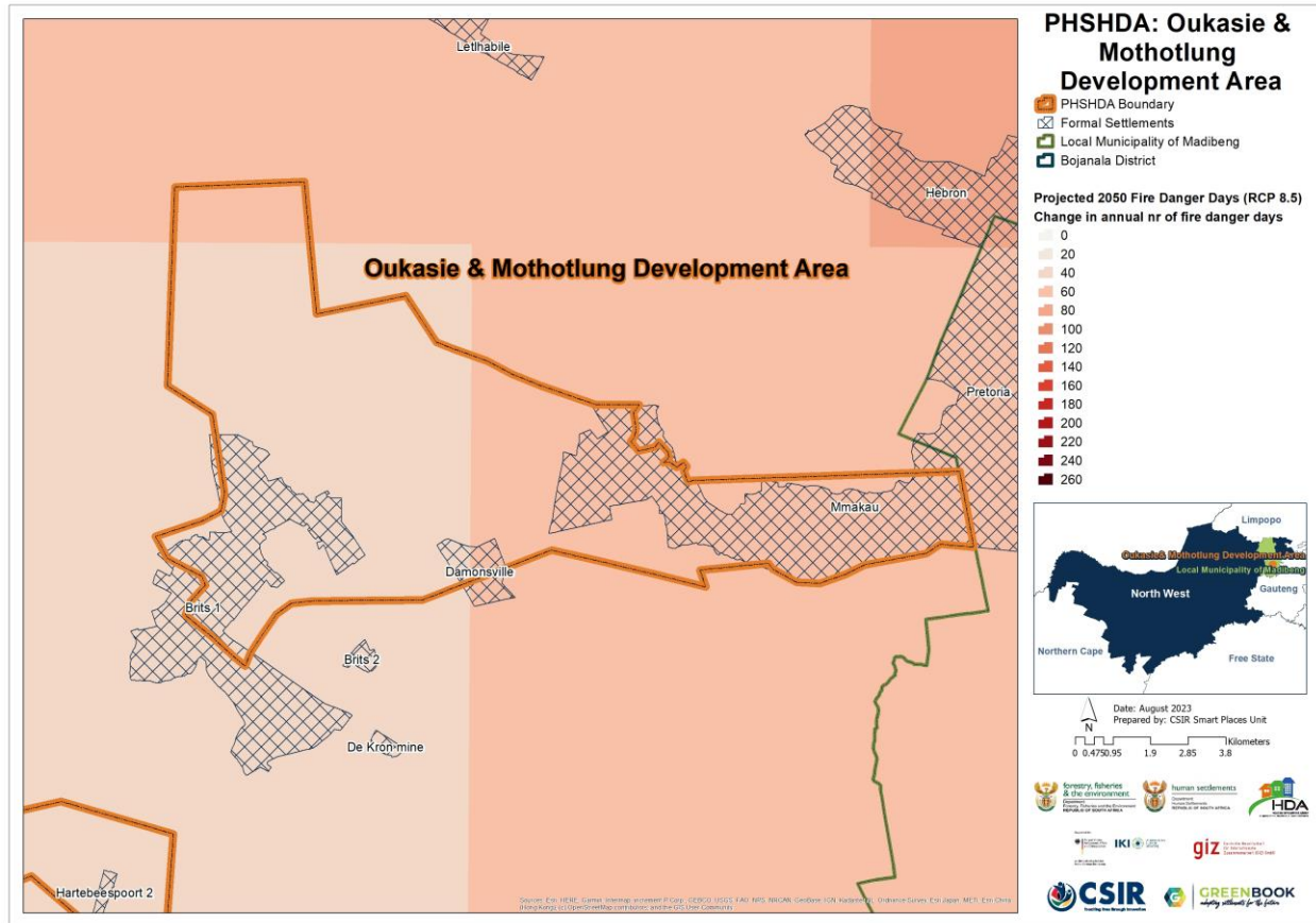
Figure 19: The number of fire danger days projected for the OM PSHDA in 2050 under the RCP 8.5 scenario.
