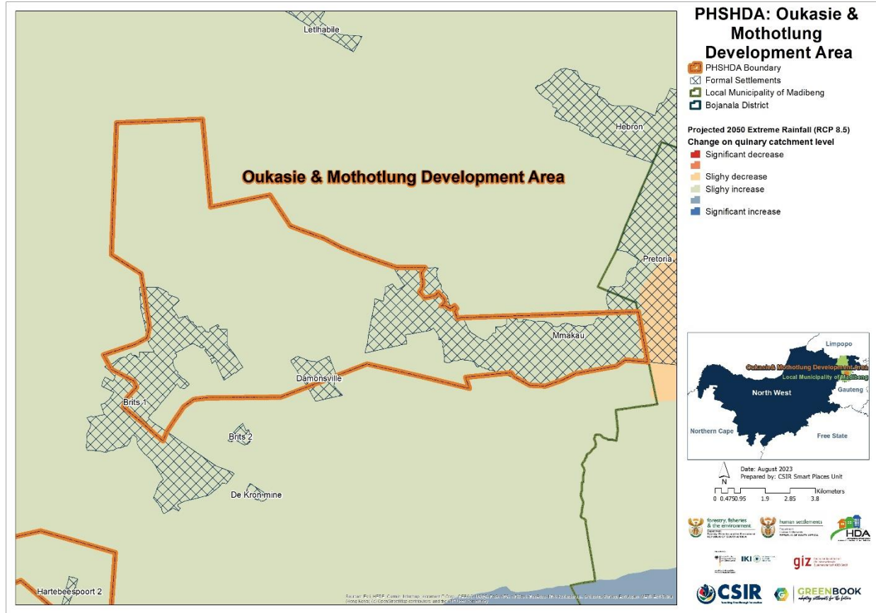
Figure 21: Projected change into the future in extreme rainfall days across OM PSHDA
