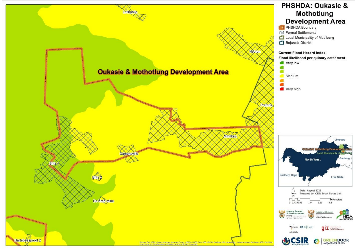
Figure 20: The flood hazard index across OM PSHDA under current (baseline) climatic conditions
