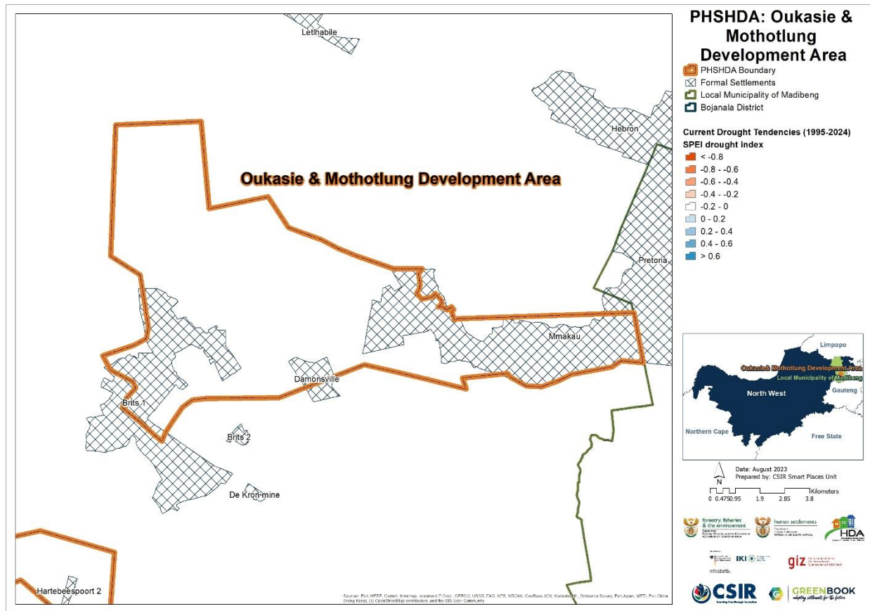
Figure 9: Projected changes in drought tendencies from the baseline period (1986 – 2005) to the current period (1995 – 2024) across OM PSHDA
