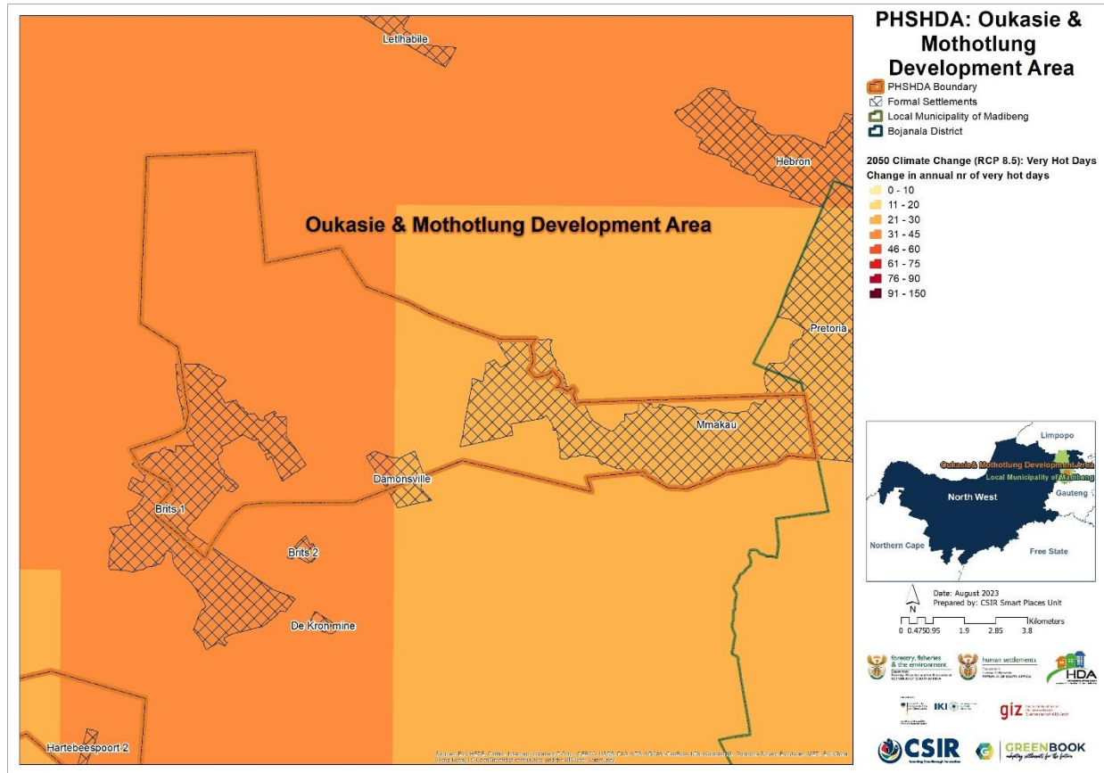
Figure 13: Projected change in annual number of very hot days across OM PSHDA with daily temperature maxima exceeding 35 °C, assuming an (RCP 8.5) emissions pathway.
