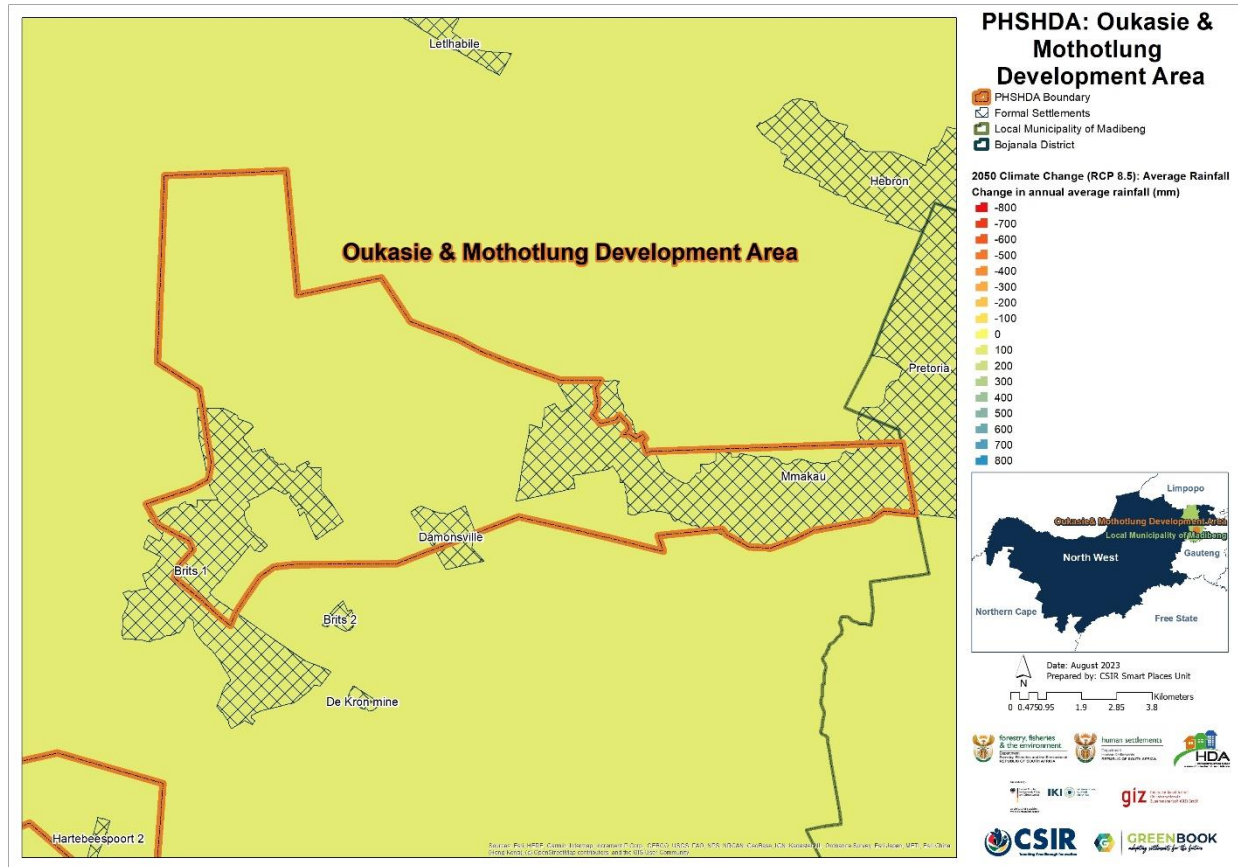
Figure 8: Projected change in average annual rainfall (mm) from the baseline period to the period 2021 – 2050 for OM PSHDA, assuming an (RCP 8.5) emissions pathway
