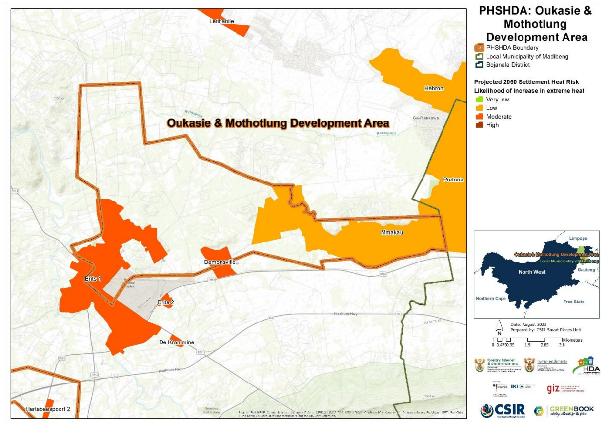
Figure 16: Heat stress risk across OM PSHDA at settlement level in the 2050s
