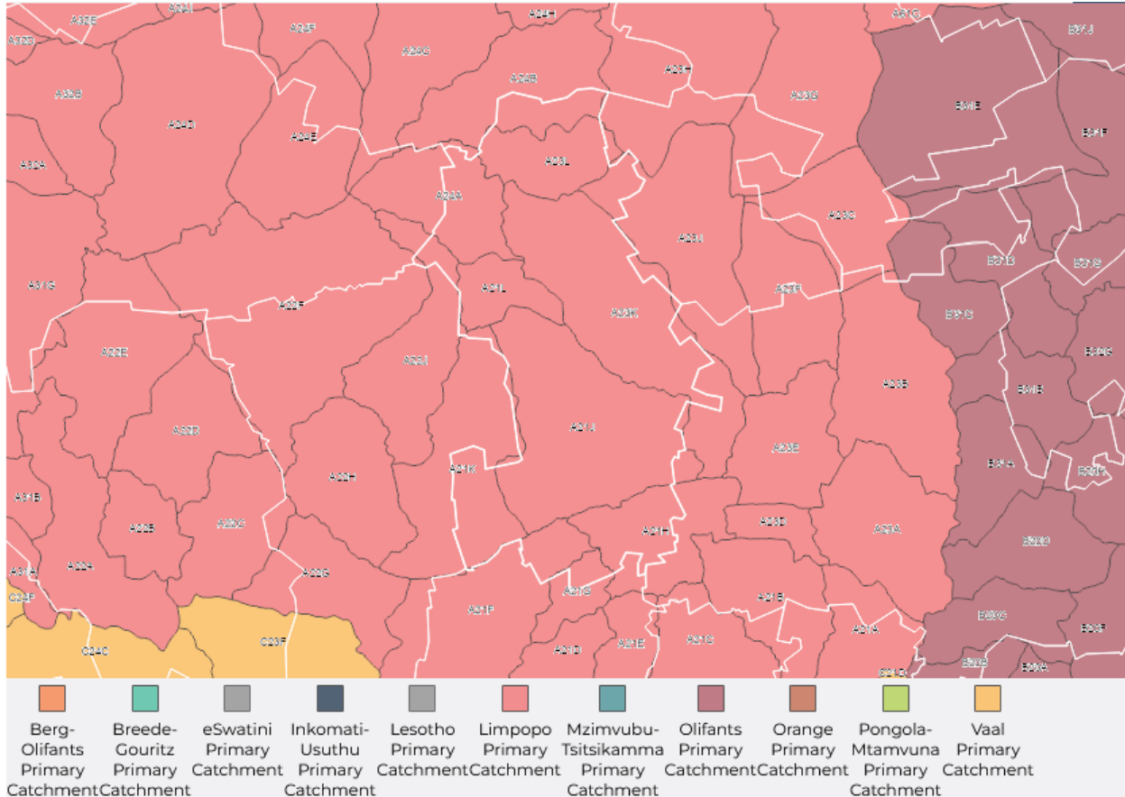
Figure 24: Quaternary catchments found in Madibeng Local Municipality
