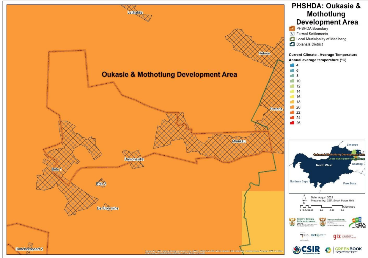
Figure 5: Average annual temperature (°C) for the baseline period 1961 – 1990 for OM PSHDA
