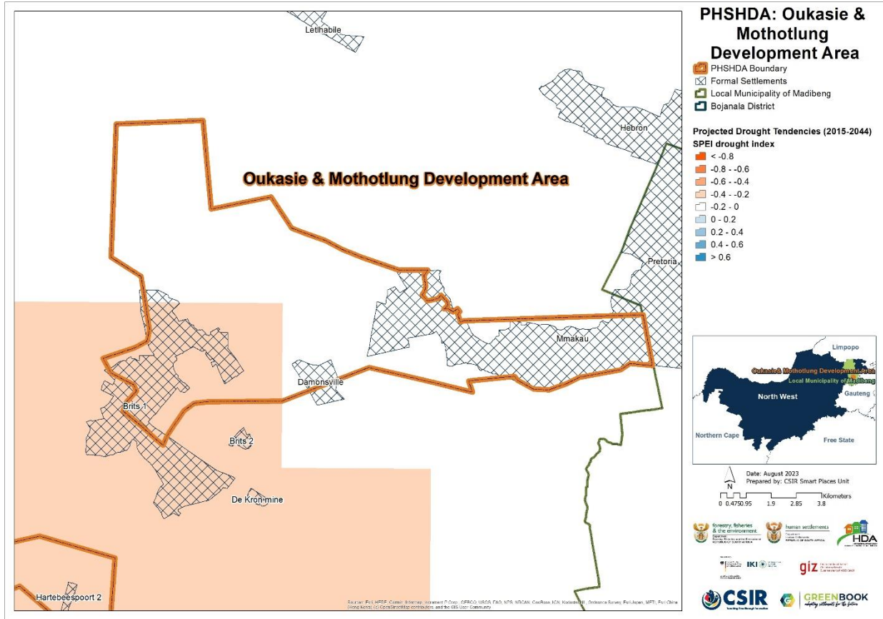
Figure 10: Projected changes in drought tendencies from the baseline period (1986 – 2005) to the future period (2015 – 2044) for OM PSHDA
