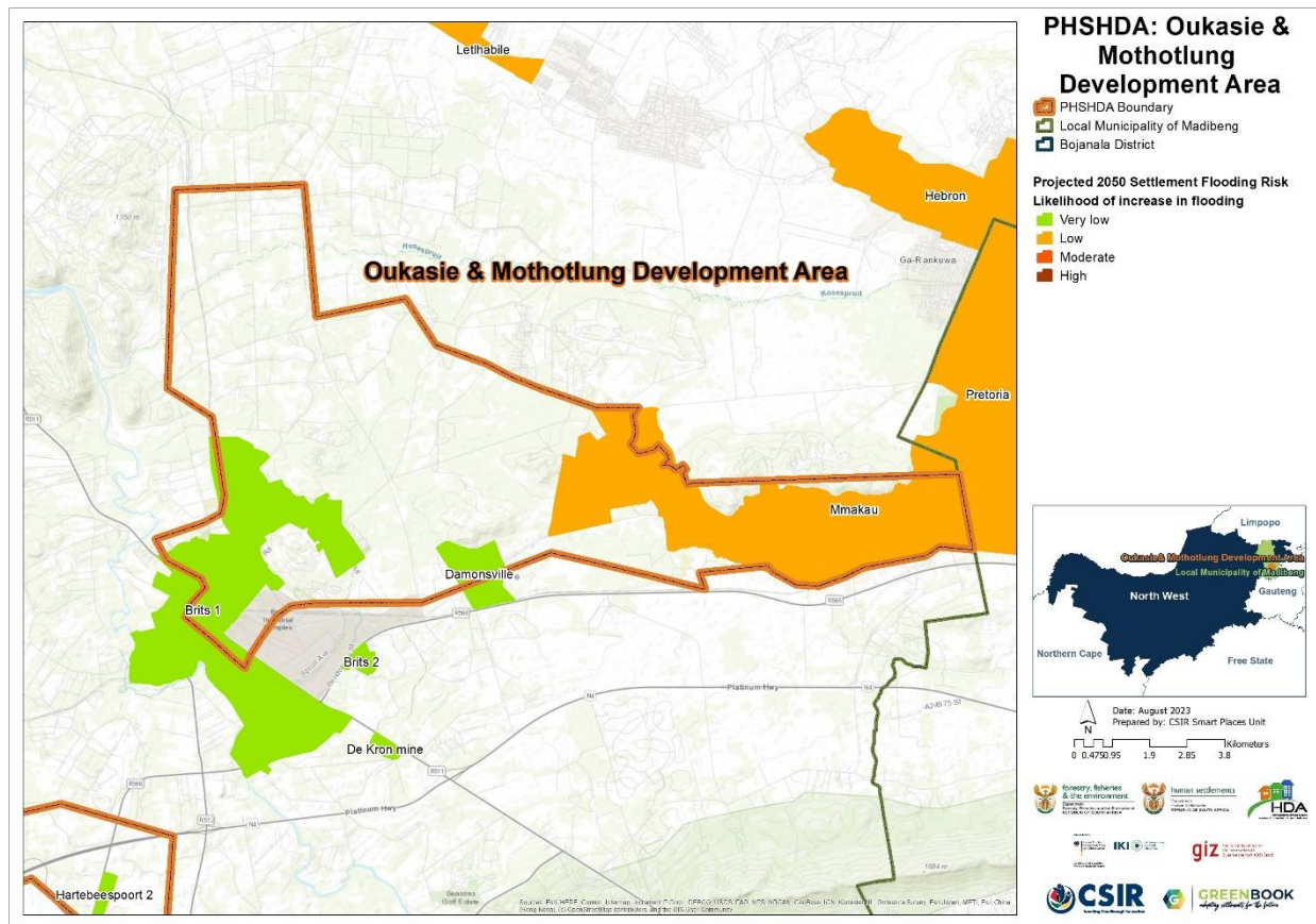
Figure 23: Flood risk into a climate change future at settlement level across OM PSHDA
