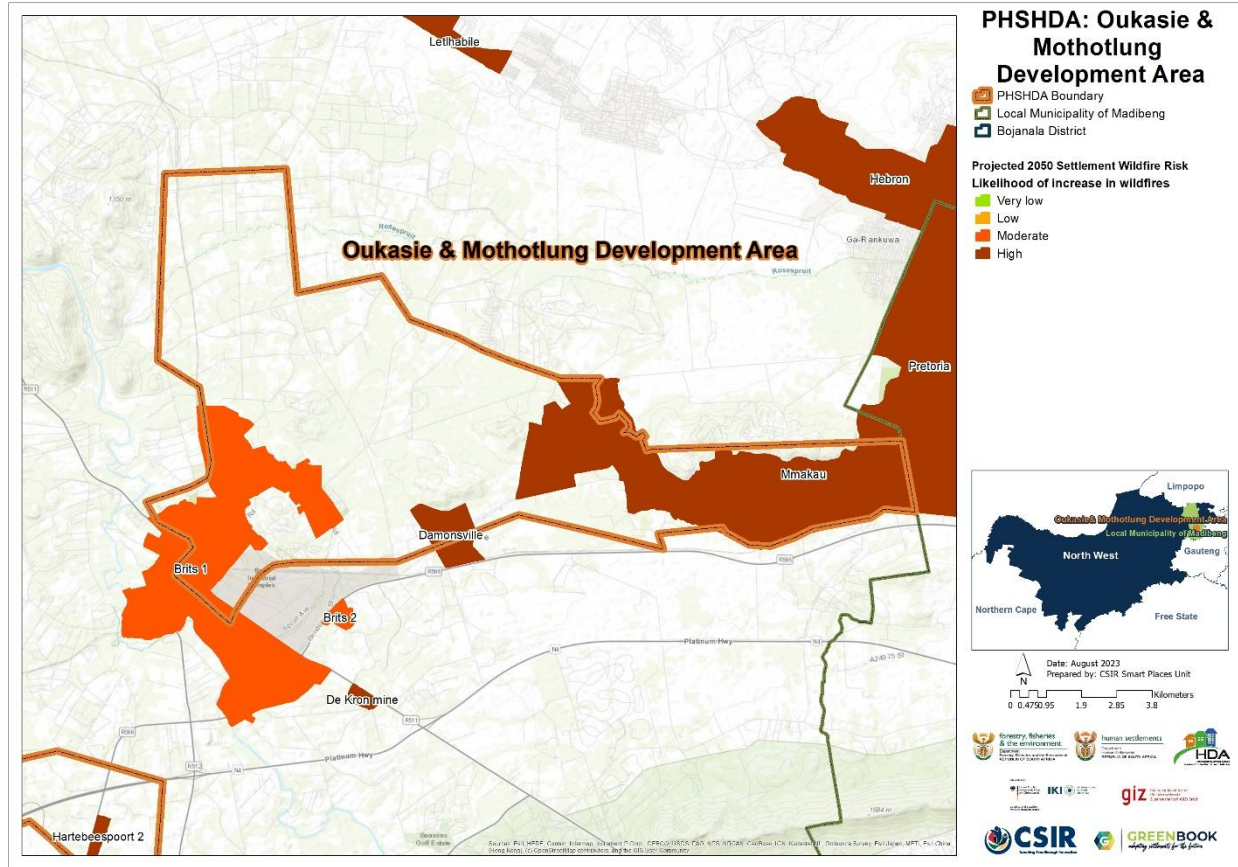
Figure 18: The likelihood of wildfires under projected climatic conditions across settlements in OM PSHDA
