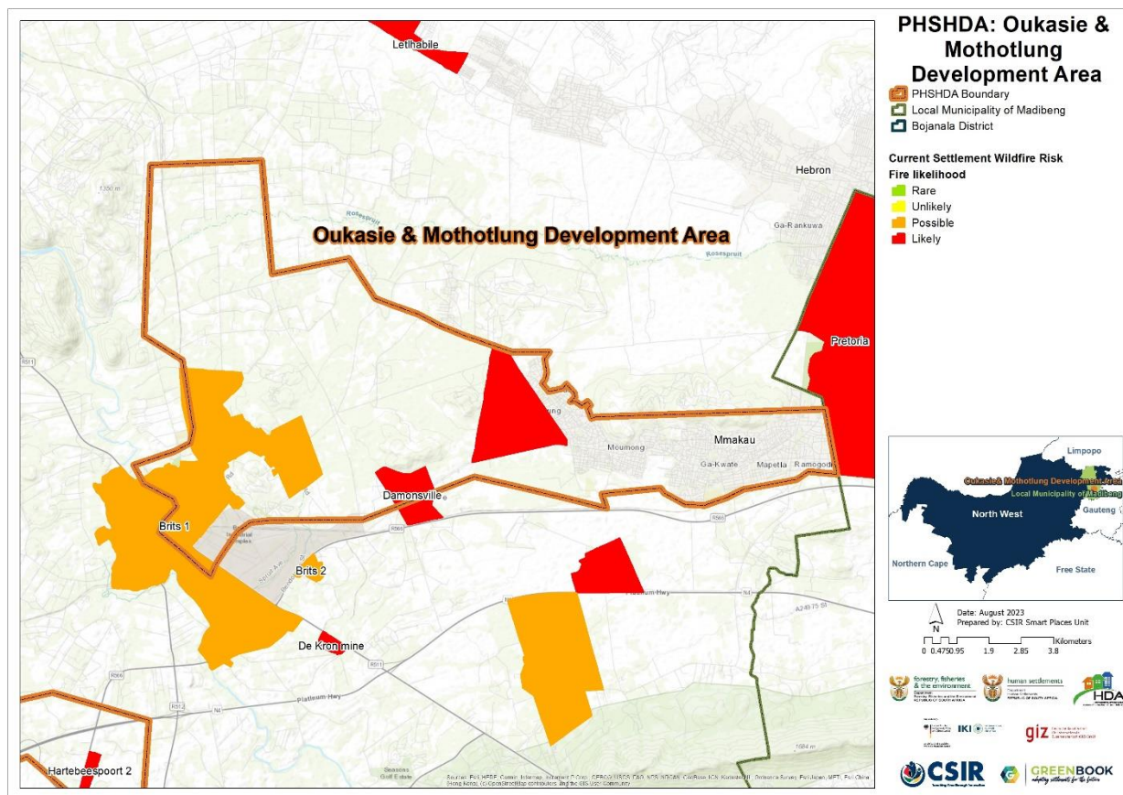
Figure 17: The likelihood of wildfires under current climatic conditions across settlements in OM PSHDA
