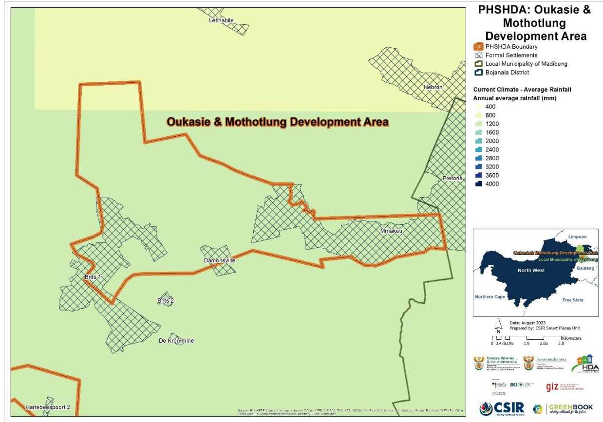
Figure 7: Average annual rainfall (mm) for the baseline period 1961 – 1990 for OM PSHDA
