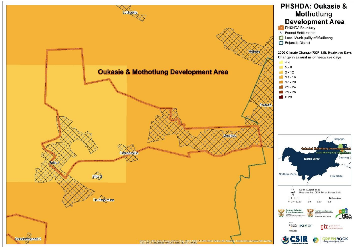
Figure 15: Projected change in annual number of heatwave days across OM PSHDA, assuming an (RCP 8.5) emissions pathway
