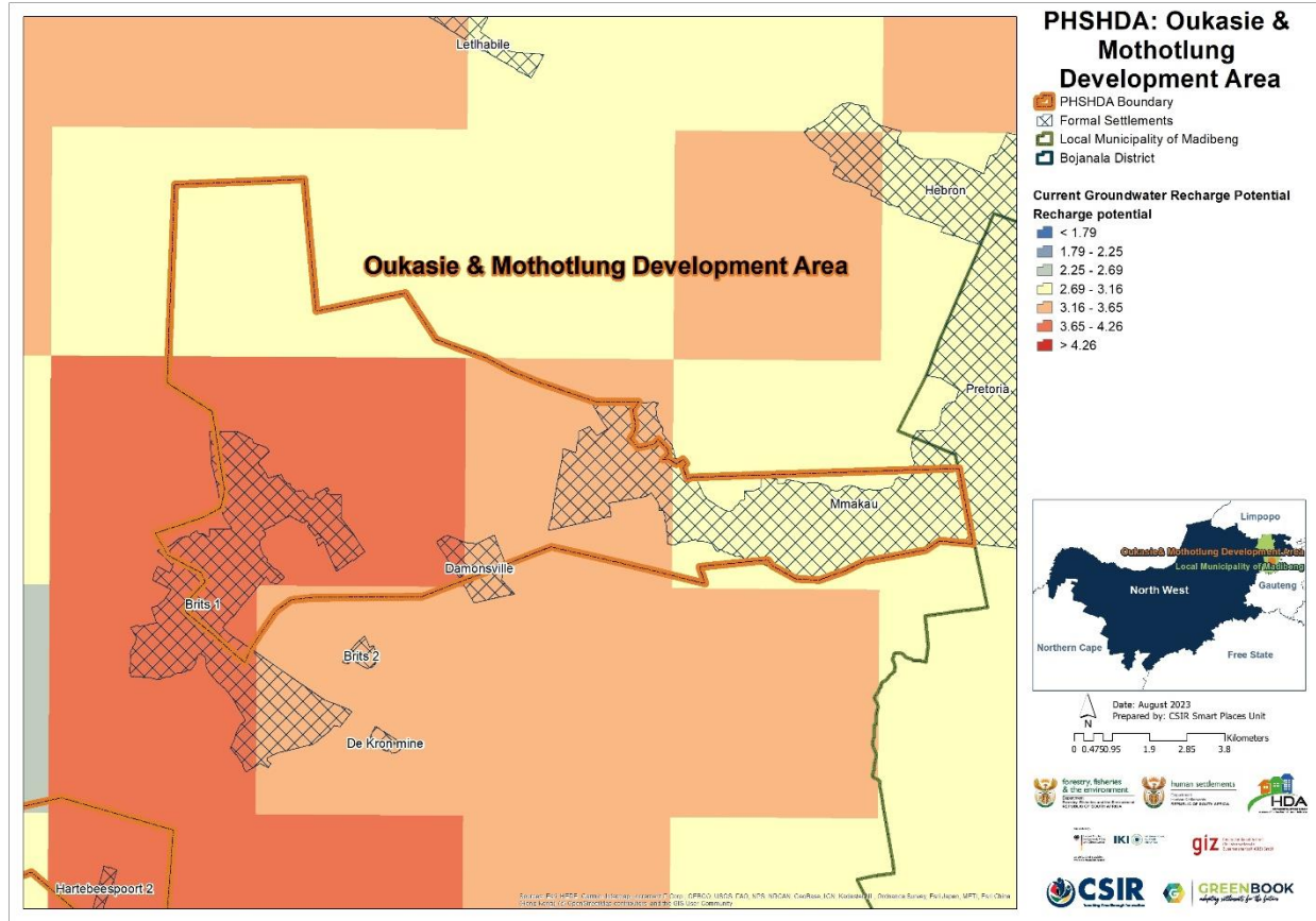
Figure 26: Groundwater recharge potential across OM PSHDA under current (baseline) climatic conditions
