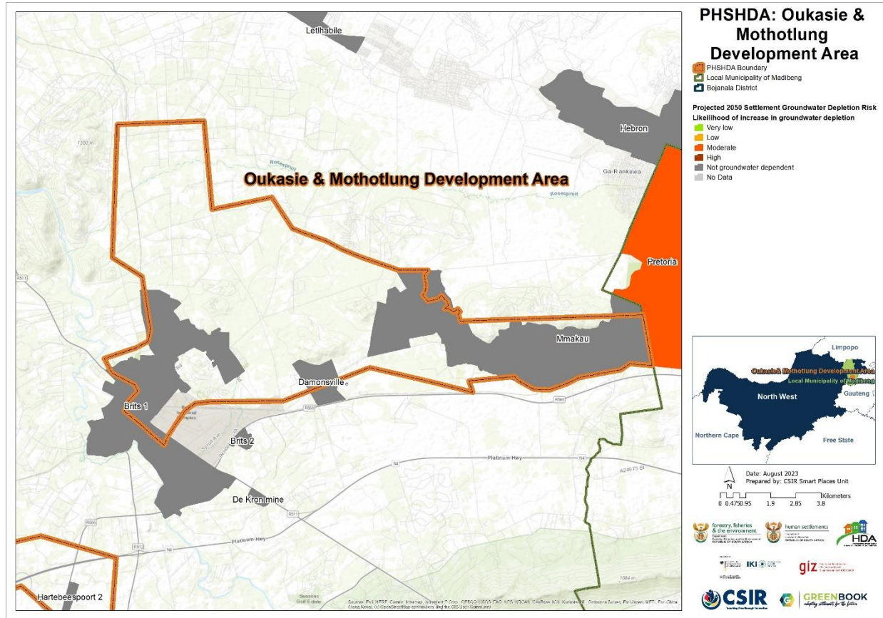
Figure 28: Settlement-level groundwater depletion across OM PSHDA
