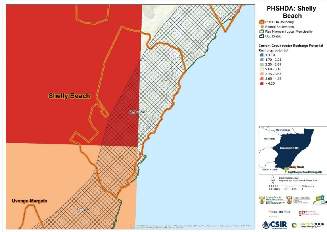
Figure 23: Groundwater recharge potential for Shelly Beach under current (baseline) climatic conditions
