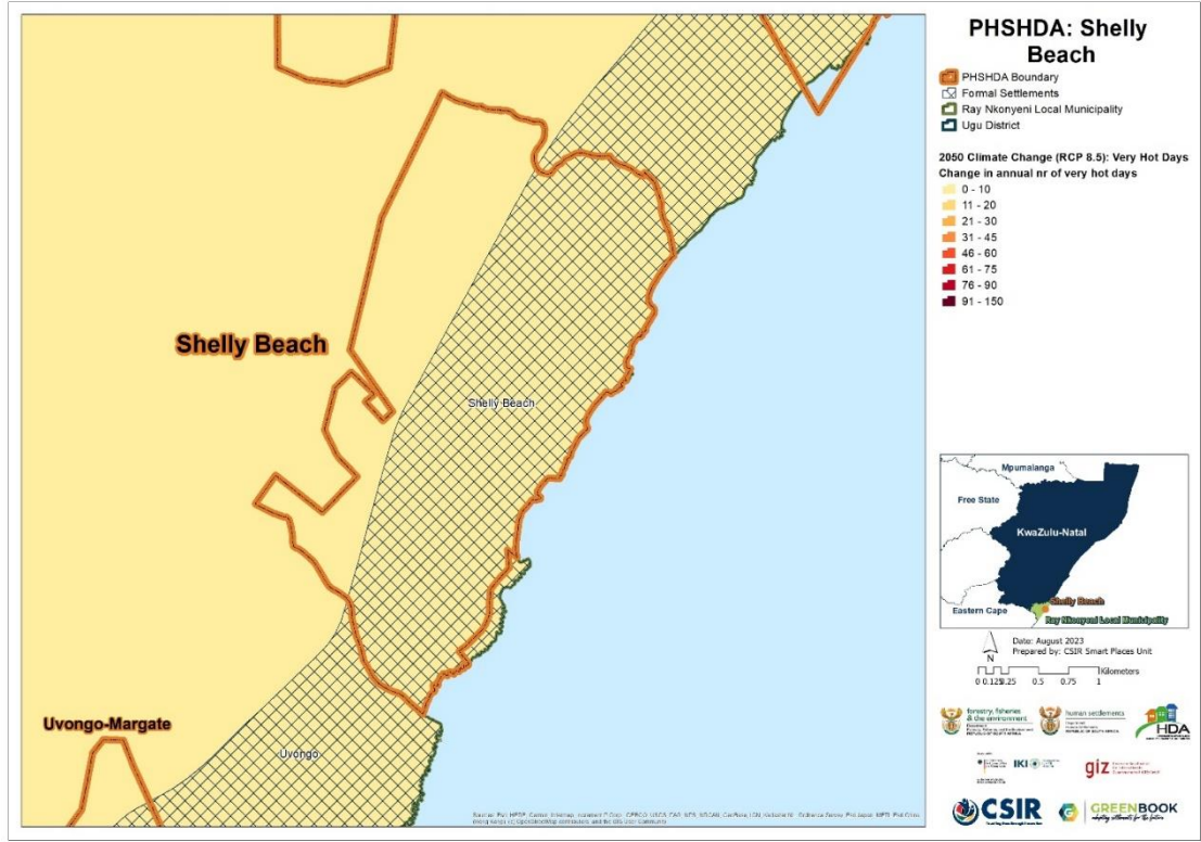
Figure 10: Projected change in annual number of very hot days for Shelly Beach with daily temperature maxima exceeding 35 °C, assuming an (RCP 8.5) emissions pathway
