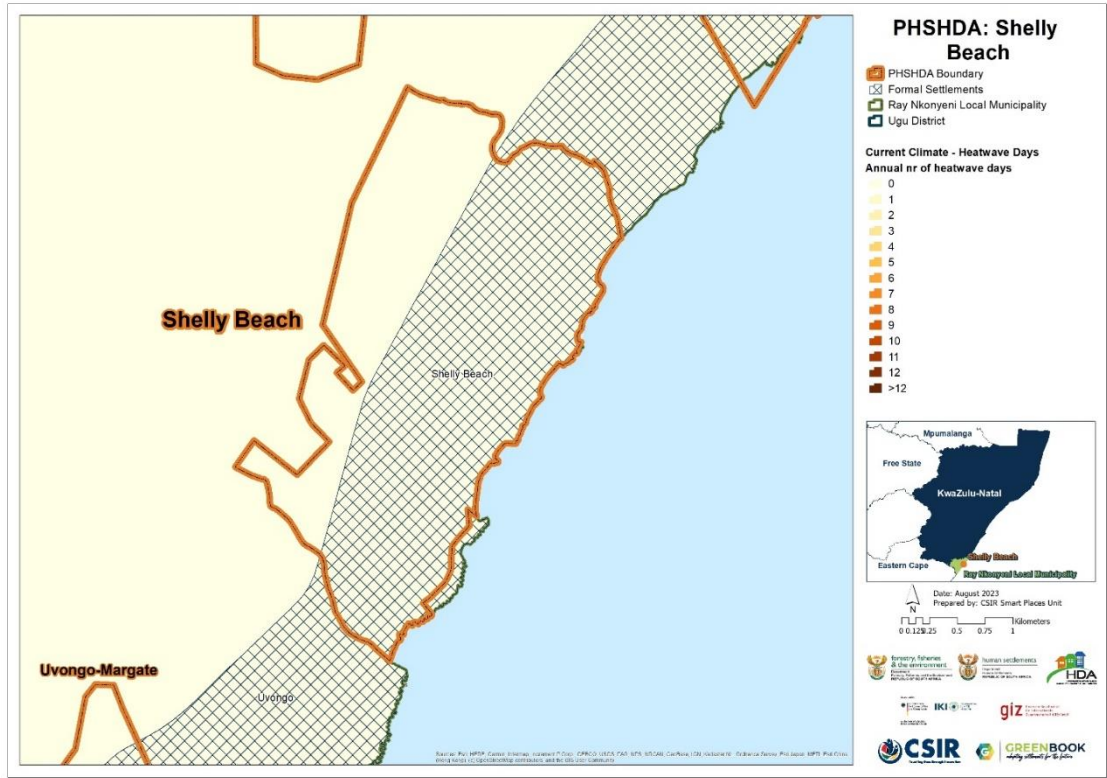
Figure 11: Annual number of heatwave days under baseline climatic conditions for Shelly Beach
