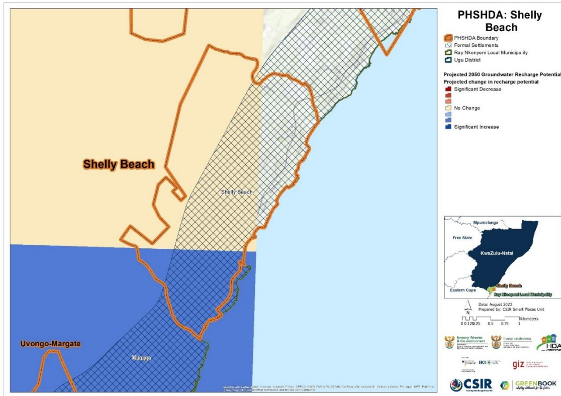
Figure 24: Projected changes in groundwater recharge potential from baseline climatic conditions to the future across Shelly Beach
