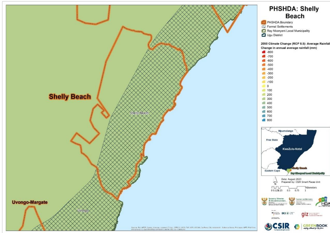
Figure 7: Projected change in average annual rainfall (mm) from the baseline period to the period 2021 – 2050 for Shelly Beach, assuming an (RCP 8.5) emissions pathway
