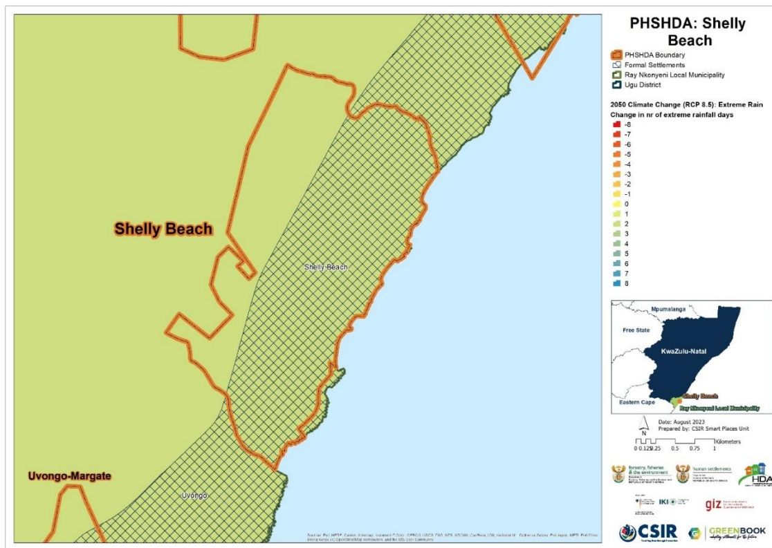
Figure 17: Projected change into the future in extreme rainfall days for Shelly Beach
