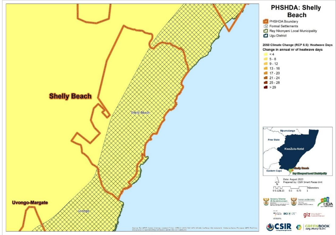
Figure 12: Projected change in annual number of heatwave days for Shelly Beach, assuming an (RCP 8.5) emissions pathway
