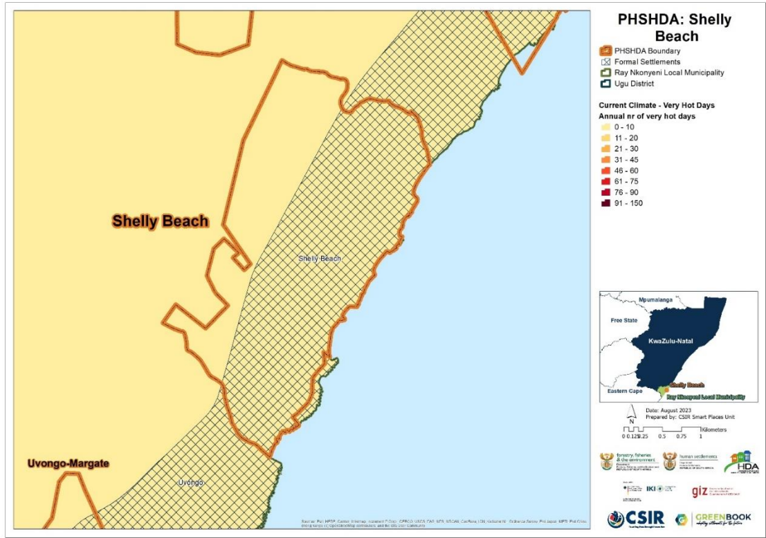
Figure 9: Annual number of very hot days under baseline climatic conditions for Shelly Beach with daily temperature maxima exceeding 35 °C
