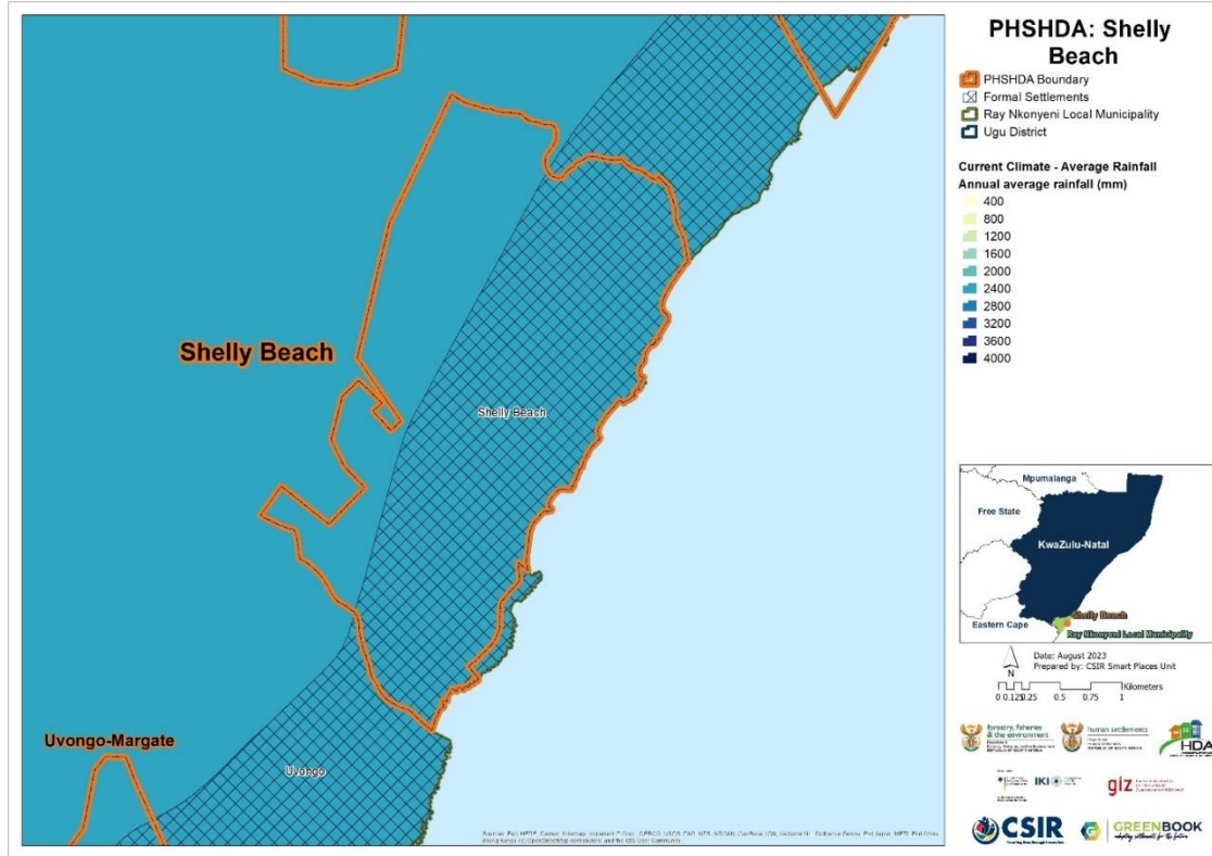
Figure 6: Average annual rainfall (mm) for the baseline period 1961 – 1990 for Shelly Beach
