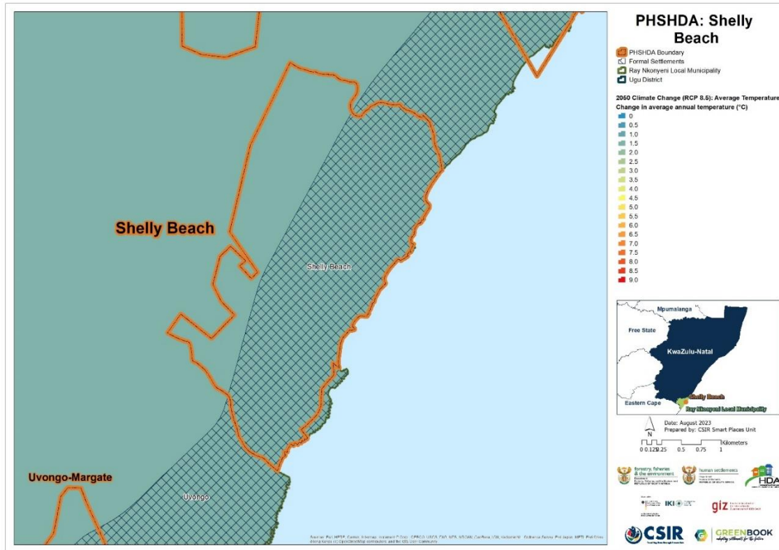
Figure 5: Projected change in average annual temperature (°C) from the baseline period to the period 2021 – 2050 for Shelly Beach, assuming an (RCP 8.5) emissions pathway
