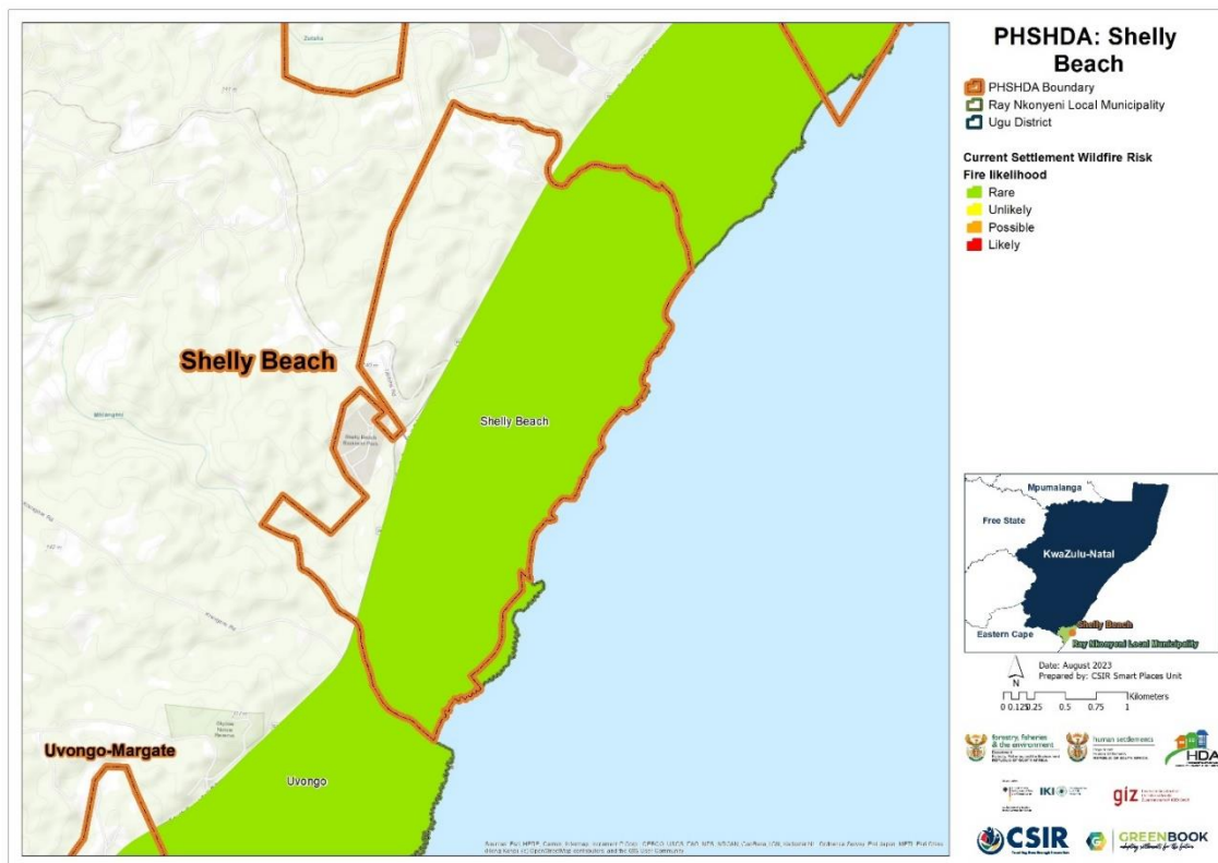
Figure 14: The likelihood of wildfires under current climatic conditions for Shelly Beach
