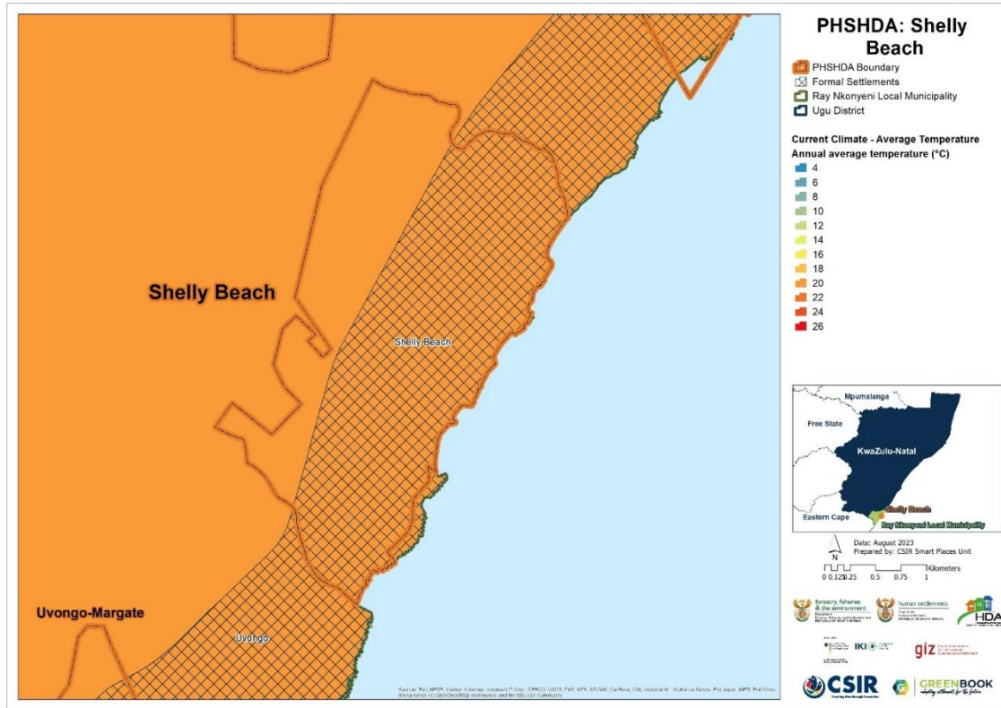
Figure 4: Average annual temperature (°C) for the baseline period 1961 – 1990 for Shelly Beach
