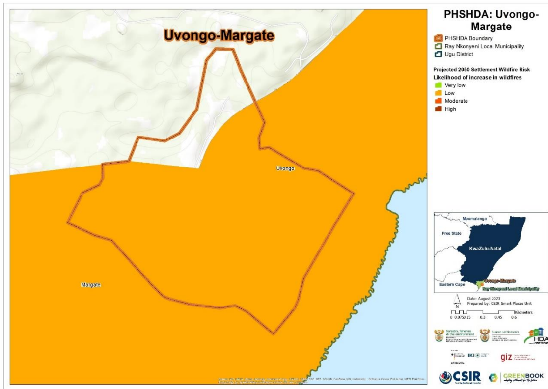
Figure 15: The likelihood of wildfires under projected climatic conditions for Uvongo-Margate
