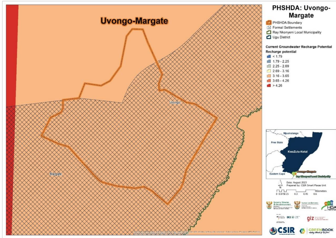
Figure 23: Groundwater recharge potential for Uvongo-Margate under current (baseline) climatic conditions
