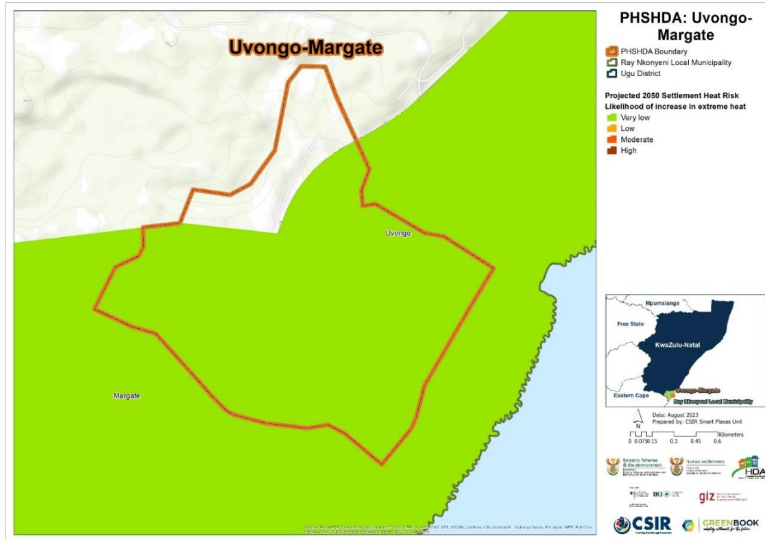
Figure 13: Heat stress risk for Uvongo-Margate at settlement level in the 2050s
