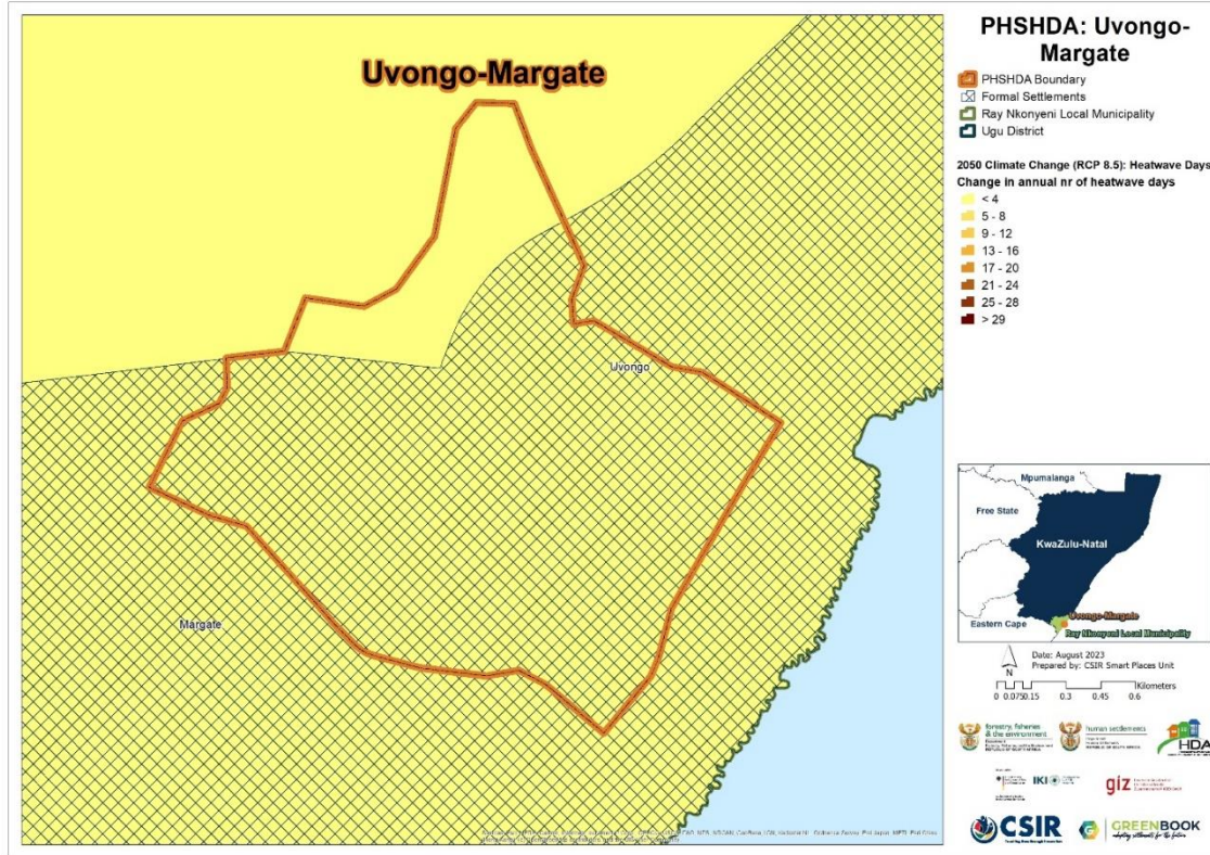
Figure 12: Projected change in annual number of heatwave days for Uvongo-Margate, assuming an (RCP 8.5) emissions pathway
