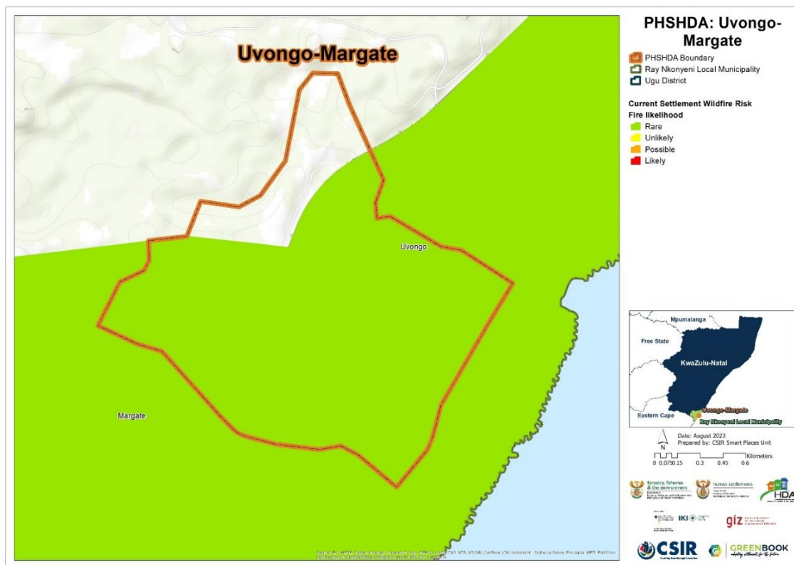
Figure 14: The likelihood of wildfires under current climatic conditions for Uvongo-Margate
