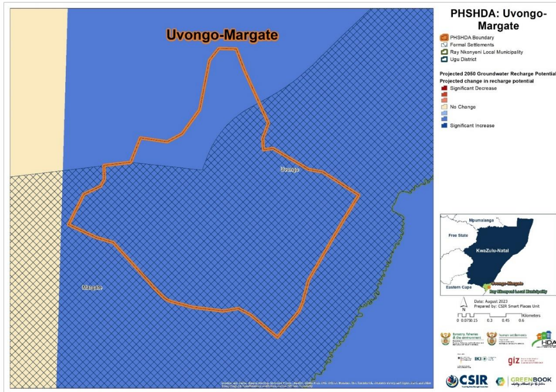
Figure 24: Projected changes in groundwater recharge potential from baseline climatic conditions to the future across Uvongo-Margate
