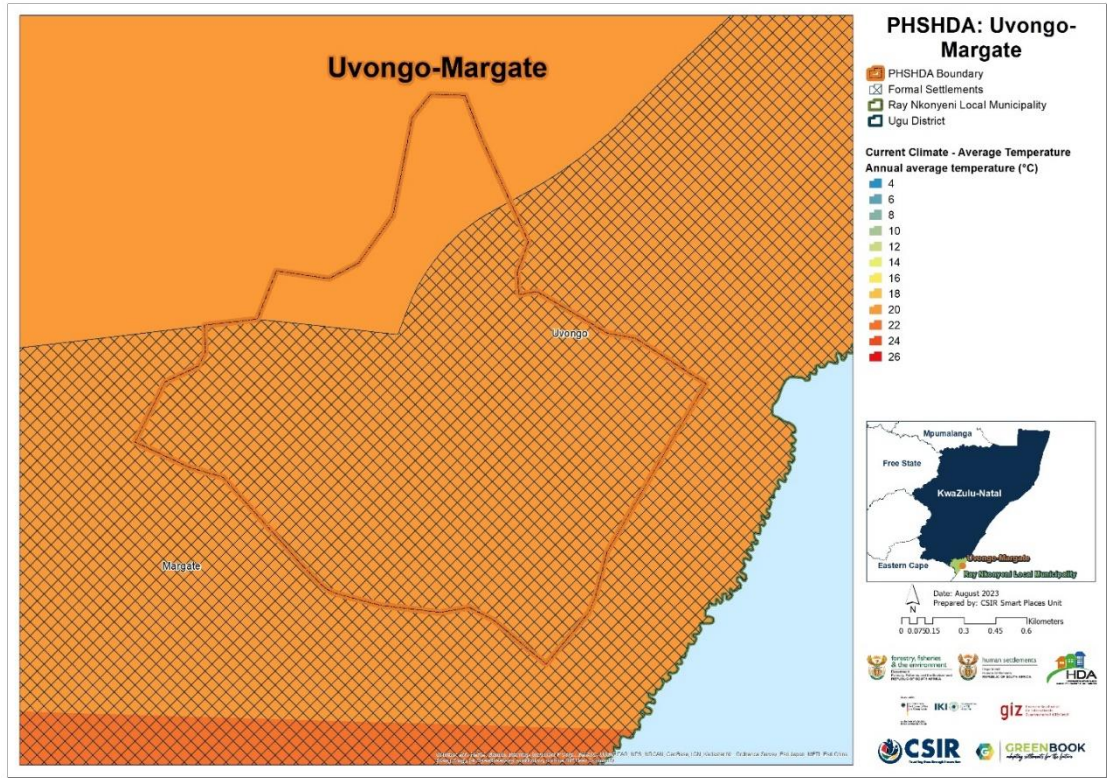
Figure 4: Average annual temperature (°C) for the baseline period 1961 – 1990 for Uvongo-Margate
