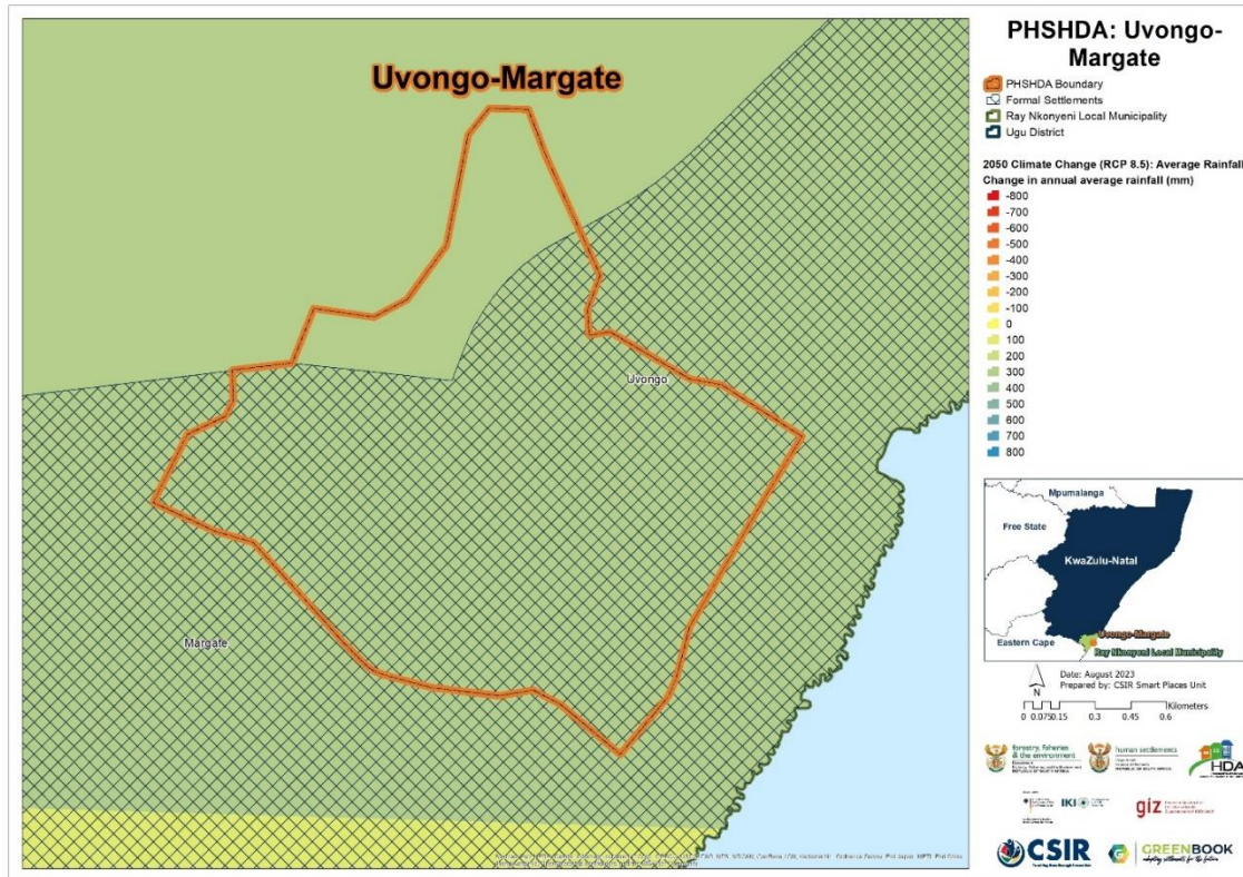
Figure 7: Projected change in average annual rainfall (mm) from the baseline period to the period 2021 – 2050 for Uvongo-Margate, assuming an (RCP 8.5) emissions pathway
