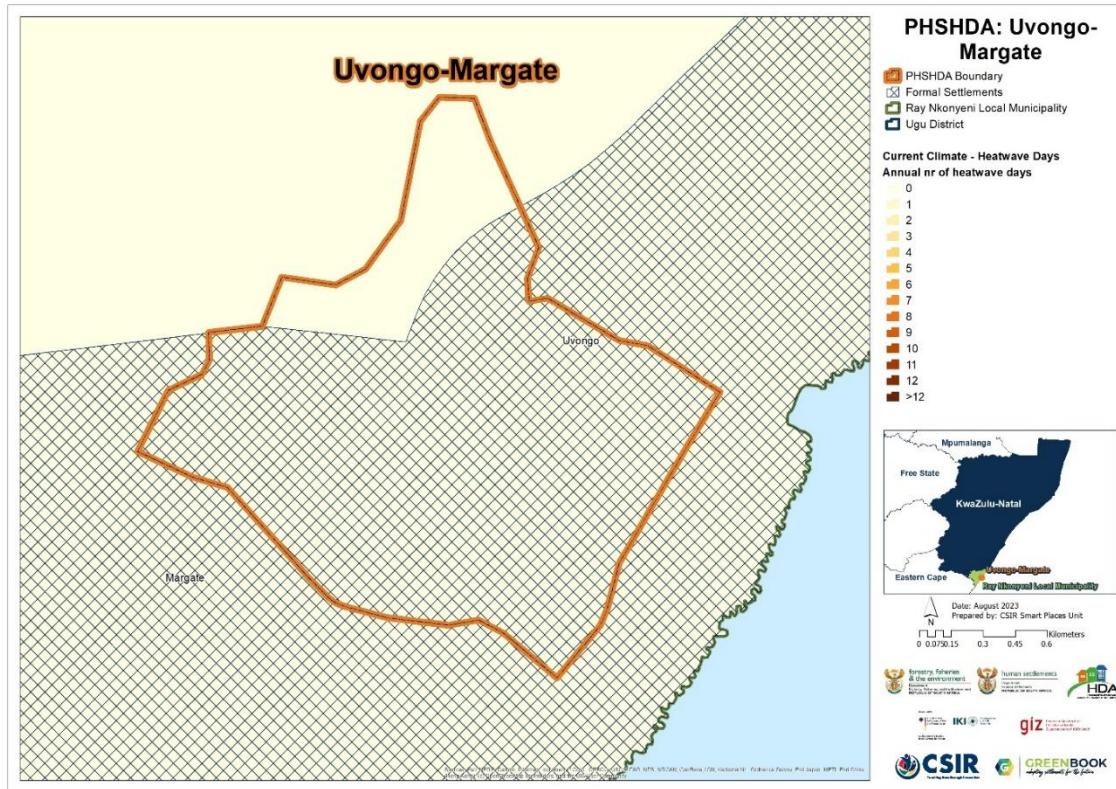
Figure 11: Annual number of heatwave days under baseline climatic conditions for Uvongo-Margate
