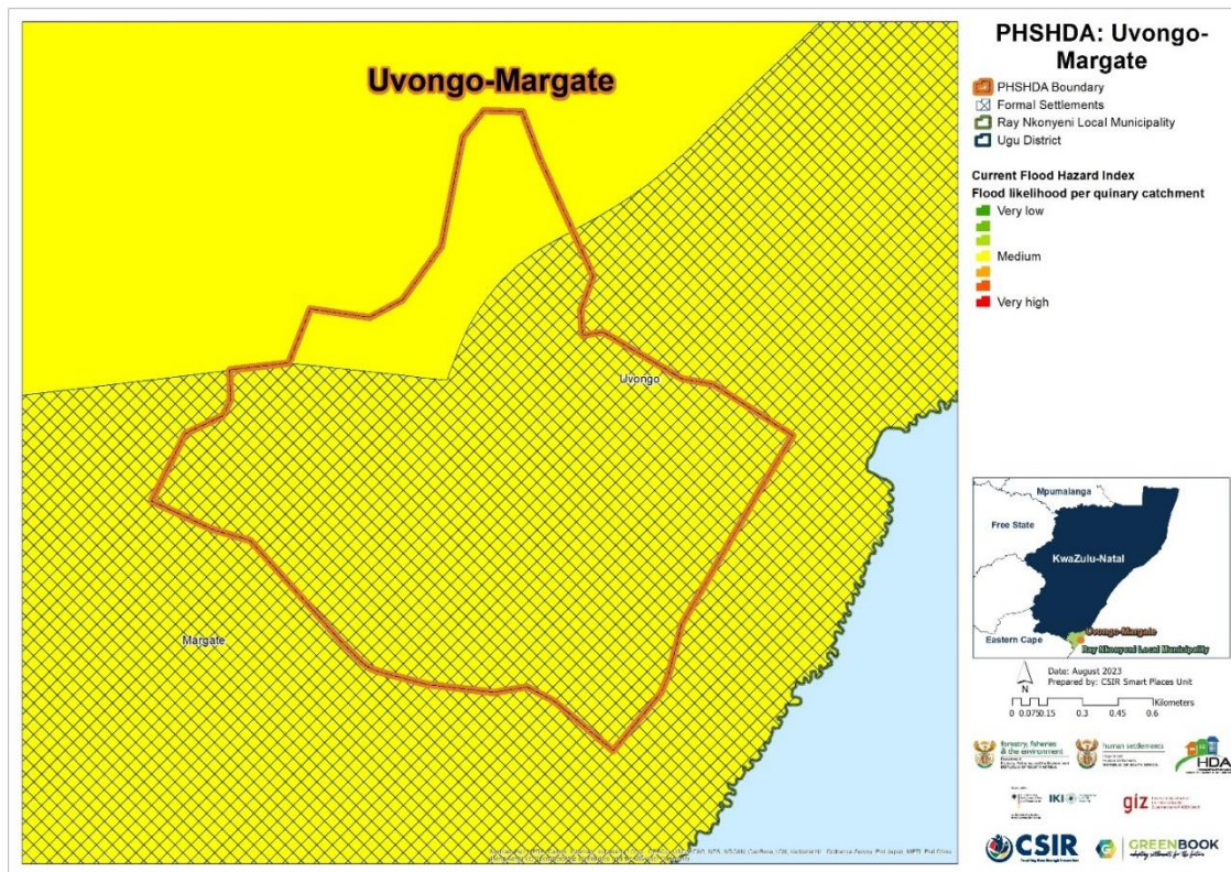
Figure 16: The flood hazard index for Uvongo-Margate under current (baseline) climatic conditions
