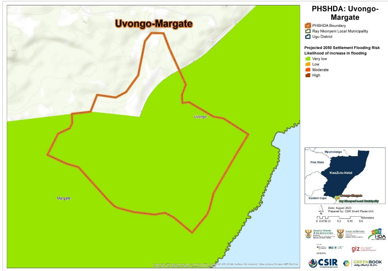
Figure 18: Flood risk into a climate change future at settlement level for Uvongo-Margate
