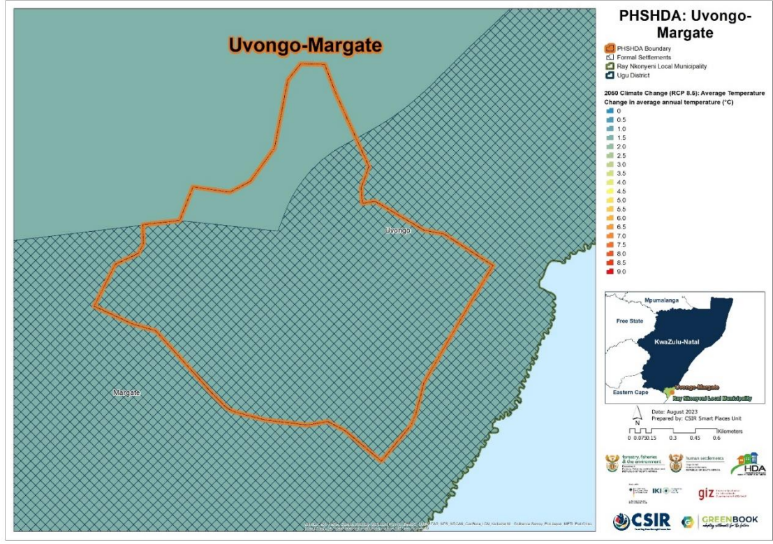
Figure 5: Projected change in average annual temperature (°C) from the baseline period to the period 2021 – 2050 for Uvongo-Margate, assuming an (RCP 8.5) emissions pathway
