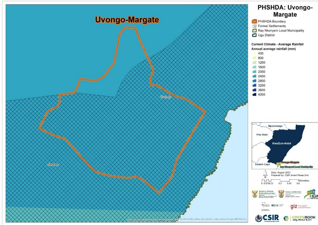
Figure 6: Average annual rainfall (mm) for the baseline period 1961 – 1990 for Uvongo-Margate
