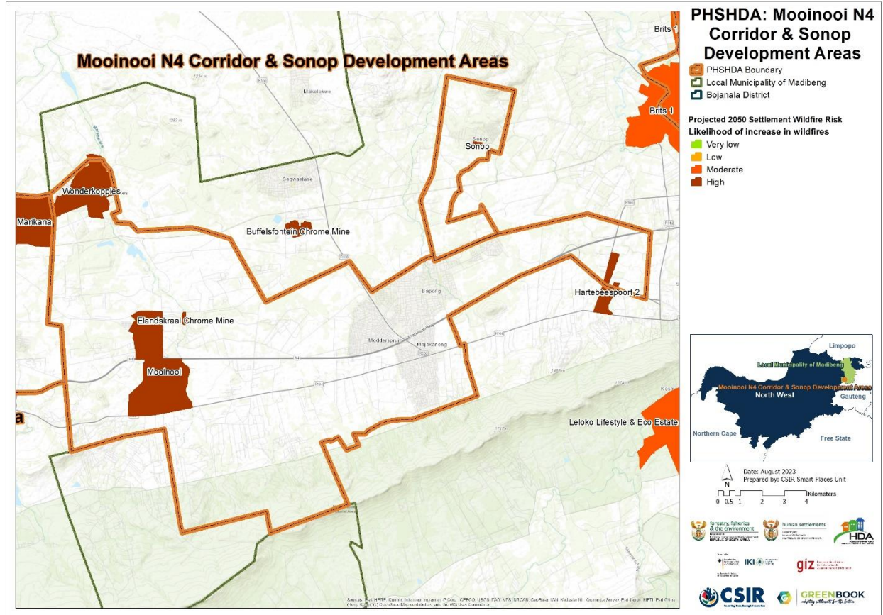
Figure 17: The likelihood of wildfires under projected climatic conditions across settlements in the MCSDA PSHDA within Madibeng Local Municipality
