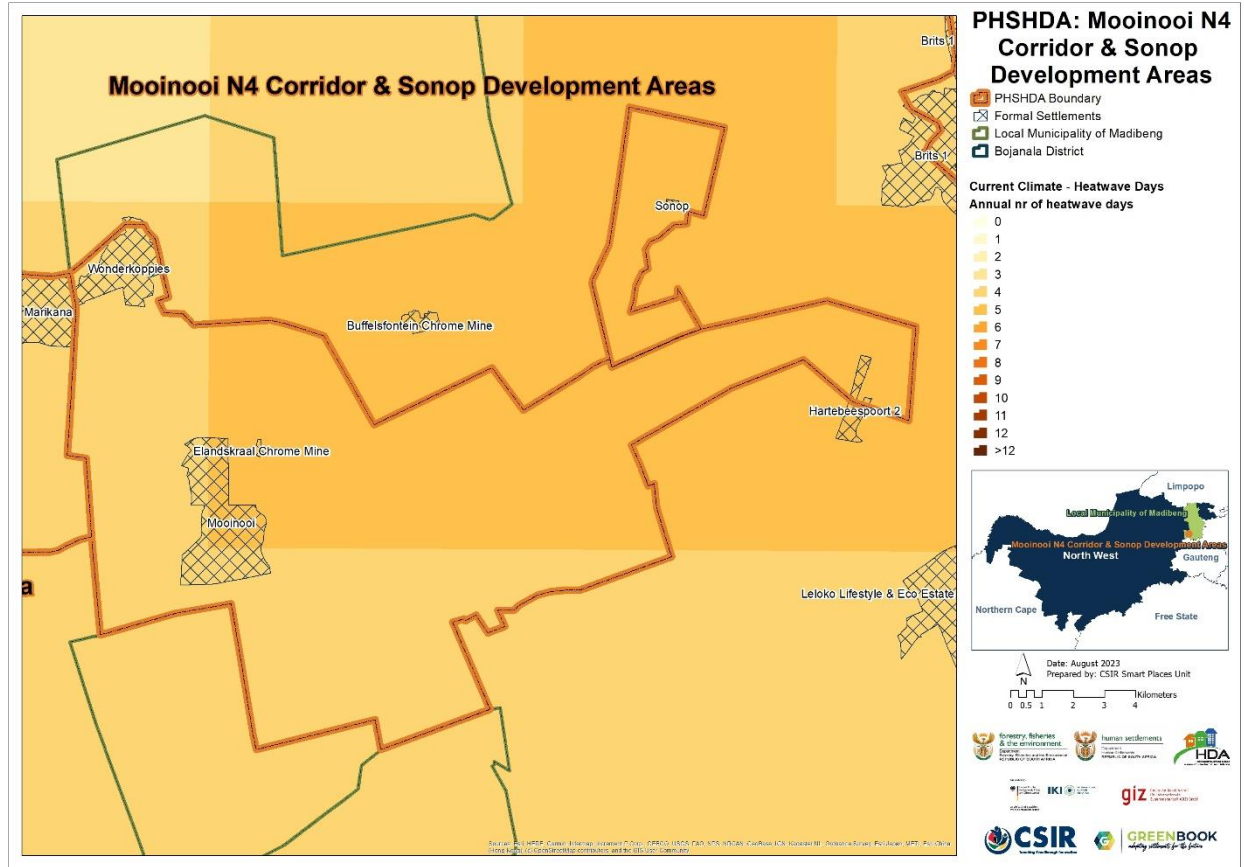
Figure 13: Annual number of heatwave days under baseline climatic conditions across the MCSDA PSHDA
