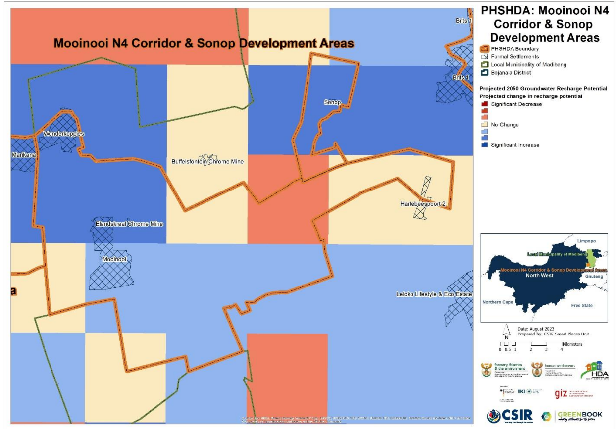
Figure 26: Projected changes in groundwater recharge potential from baseline climatic conditions to the future across MCSDA PSHDA within the Madibeng Local Municipality
