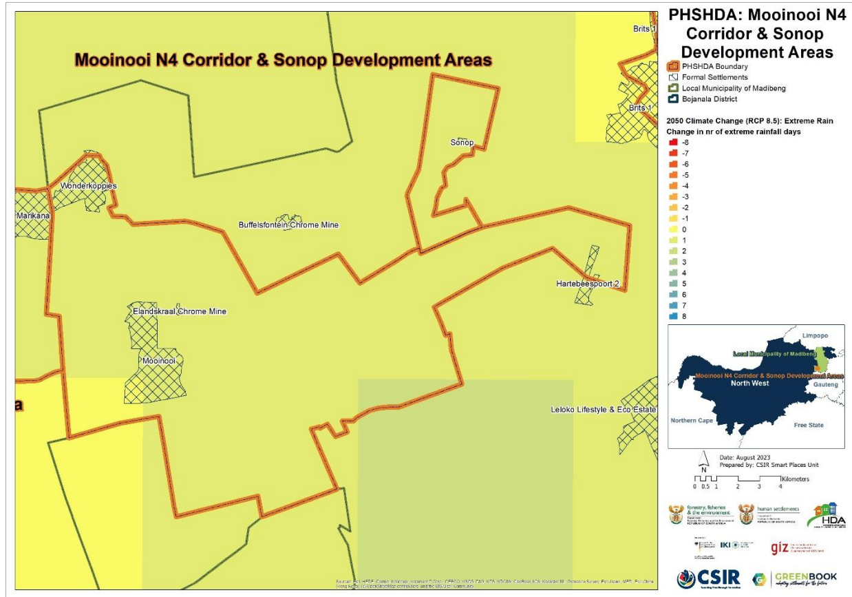
Figure 21: Projected change into the future in extreme rainfall days across the MCSDA PSHDA within the Madibeng Local Municipality.
