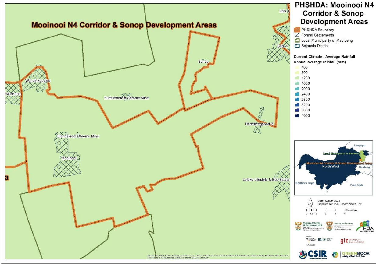
Figure 6: Average annual rainfall (mm) for the baseline period 1961 – 1990 for MCSDA PSHDA
