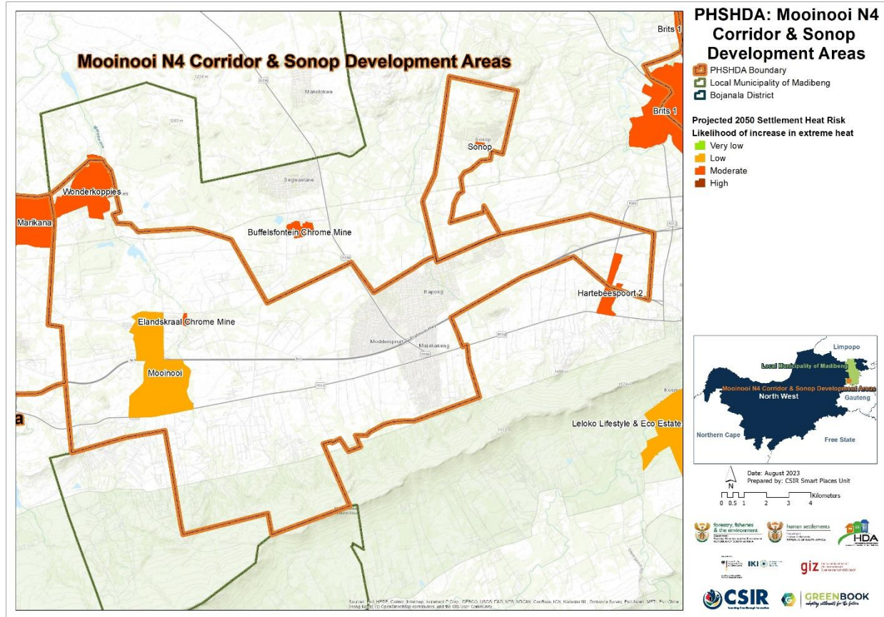
Figure 15: Heat stress risk across the MCSDA PSHDA within Madibeng Local Municipality at settlement level in the 2050s
