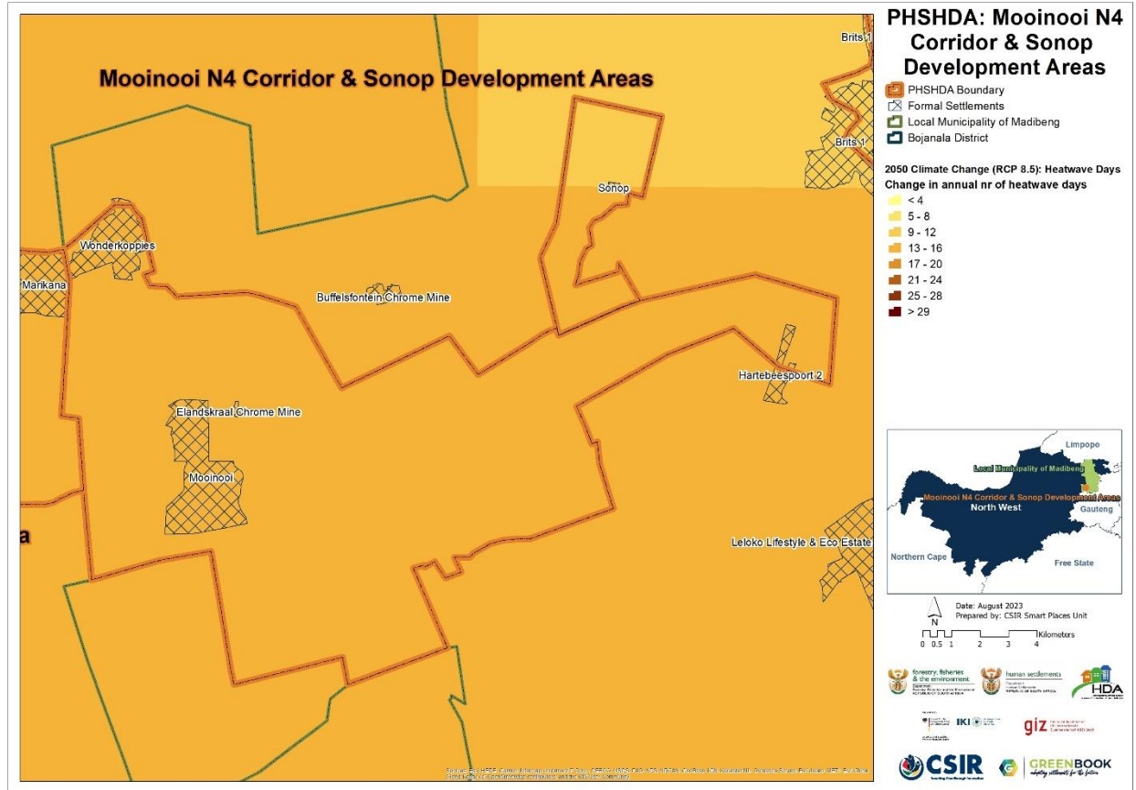
Figure 14: Projected change in annual number of heatwave days across the MCSDA PSHDA within Madibeng Local Municipality, assuming an (RCP 8.5) emissions pathway
