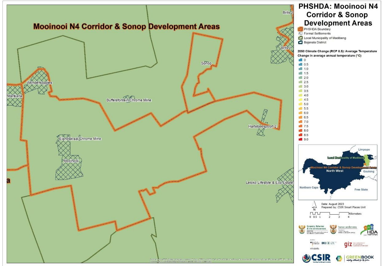
Figure 5: Projected change in average annual temperature (°C) from the baseline period to the period 2021 – 2050 for MCSDA PSHDA, assuming an (RCP 8.5) emissions pathway
