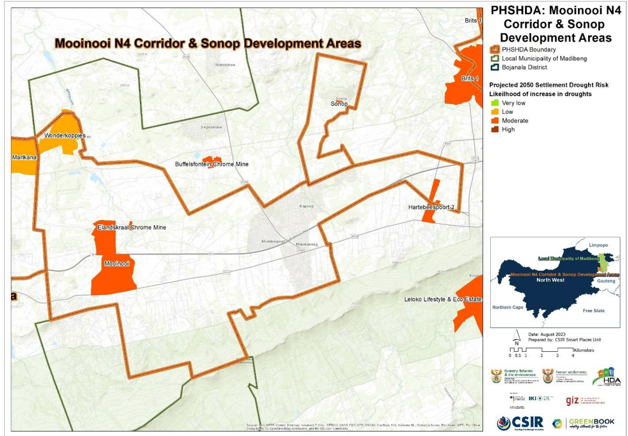
Figure 10: Settlement-level drought risk for the Mooinooi N4 Corridor and Sonop Development Areas within the Madibeng Local Municipality
