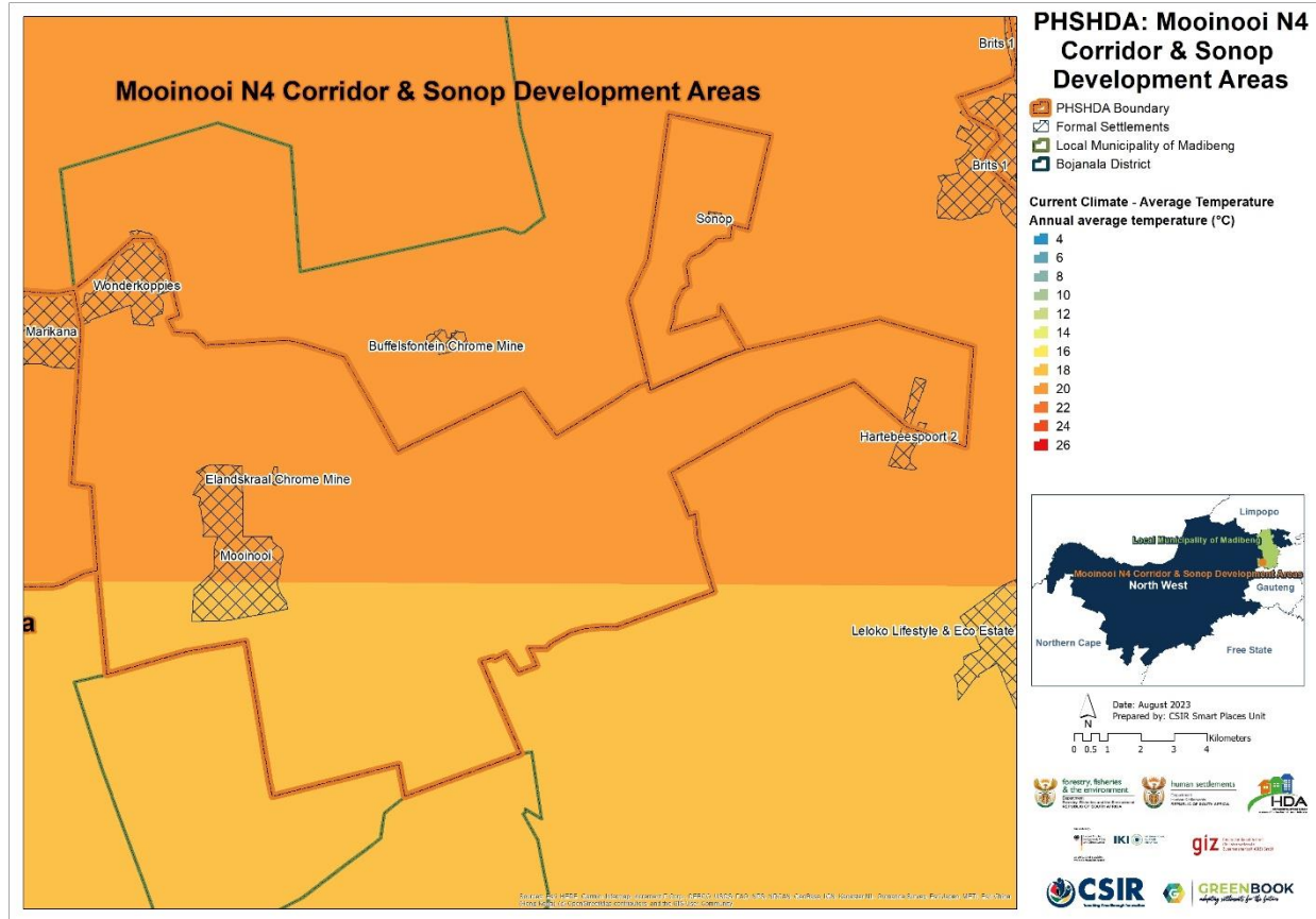
Figure 4: Average annual temperature (°C) for the baseline period 1961 – 1990 for MCSDA PSHDA
