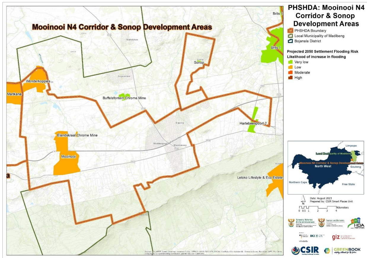
Figure 22: Flood risk into a climate change future at settlement level across the MCSDA PSHDA within the Madibeng Local Municipality
