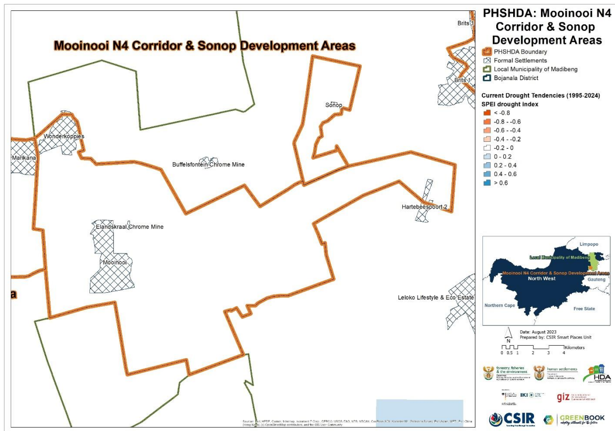
Figure 8: Projected changes in drought tendencies from the baseline period (1986 – 2005) to the current period (1995 – 2024) across the MCSDA PSHDA
