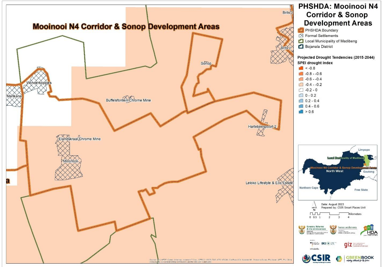
Figure 9: Projected changes in drought tendencies from the baseline period (1986 – 2005) to the future period (2015 – 2044) for MCSDA PSHDA.
