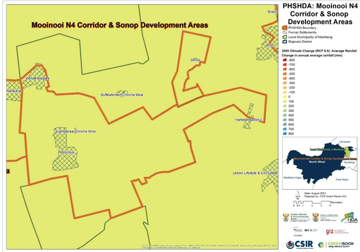
Figure 7: Projected change in average annual rainfall (mm) from the baseline period to the period 2021 – 2050 for MCSDA PSHDA, assuming an (RCP 8.5) emissions pathway
