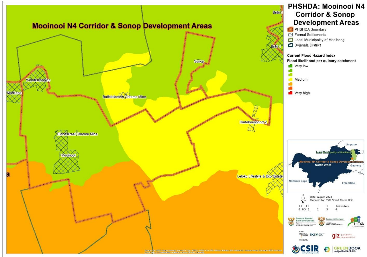
Figure 19: The flood hazard index across the MCSDA PSHDA within the Madibeng Local Municipality under current (baseline) climatic conditions
