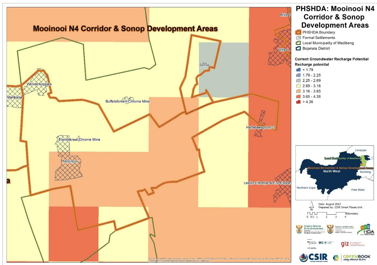
Figure 25: Groundwater recharge potential across MCSDA PSHDA within Madibeng Local Municipality under current (baseline) climatic conditions
