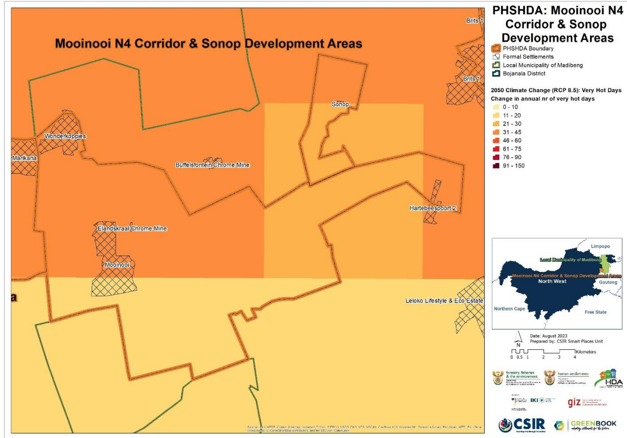
Figure 12: Projected change in annual number of very hot days across the MCSDA PSHDA with daily temperature maxima exceeding 35 °C, assuming an (RCP 8.5) emissions pathway
