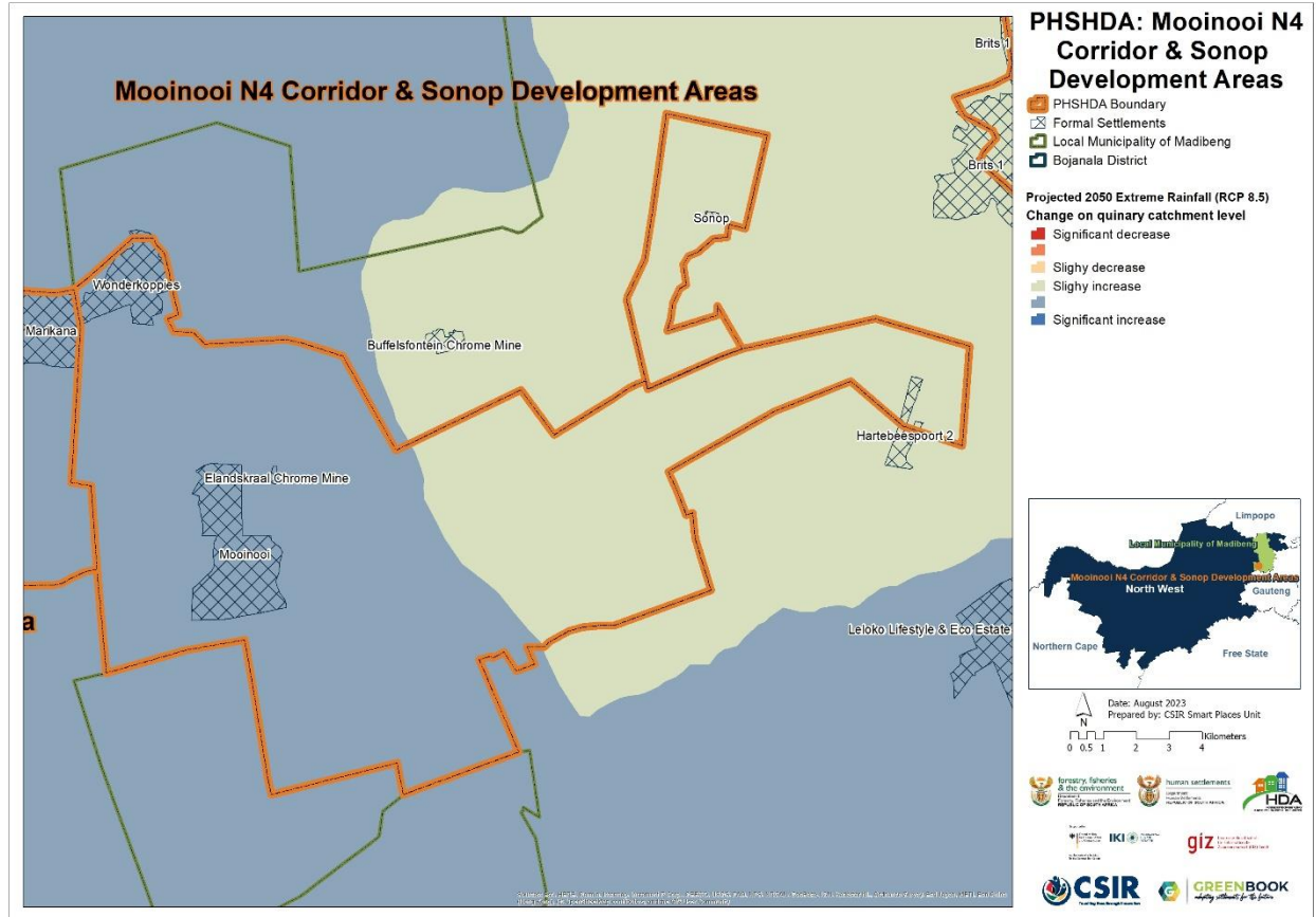
Figure 20: Projected 2050 extreme rainfall on the quinary catchment level across MCSDA PSHDA within the Madibeng Local Municipality under an RCP8.5 scenario.
