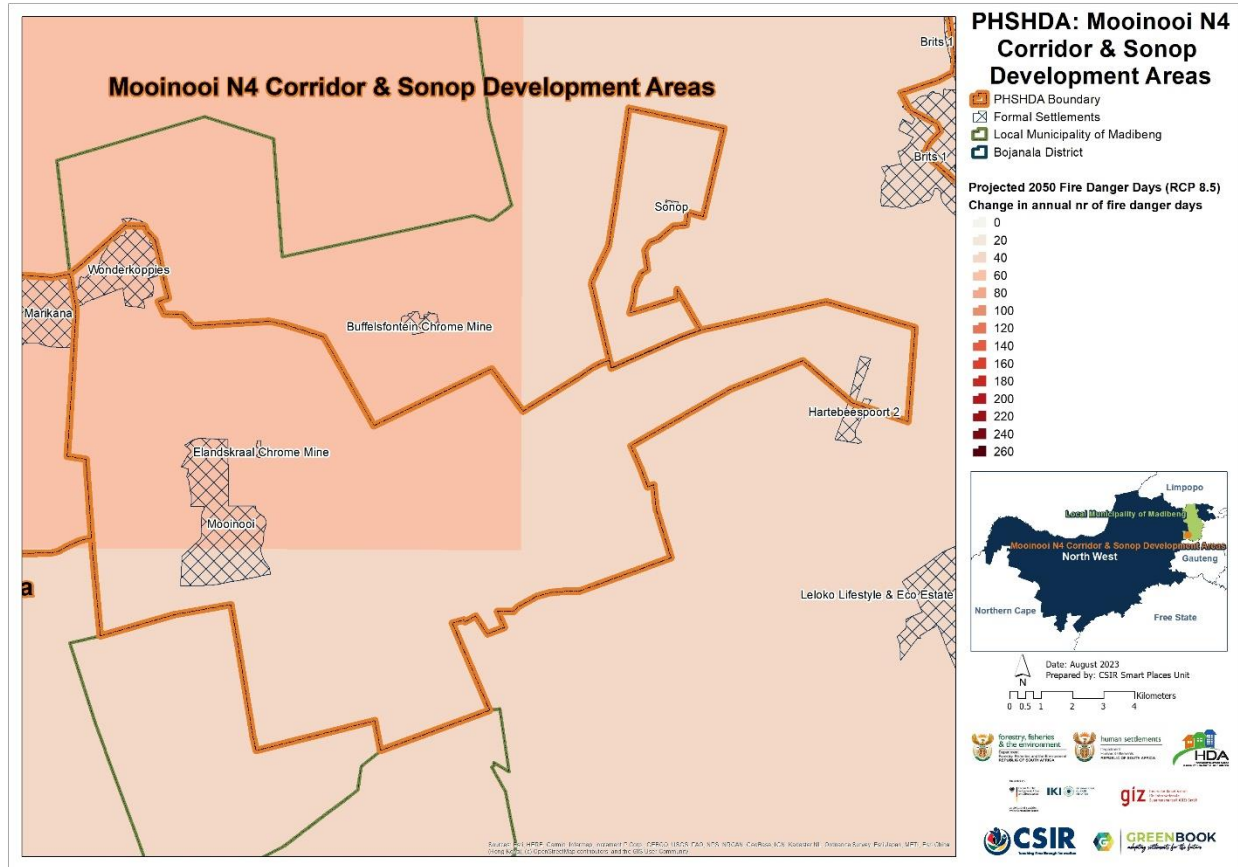
Figure 18: The number of fire danger days projected for the MCSDA PSHDA in 2050 under the RCP 8.5 scenario.
