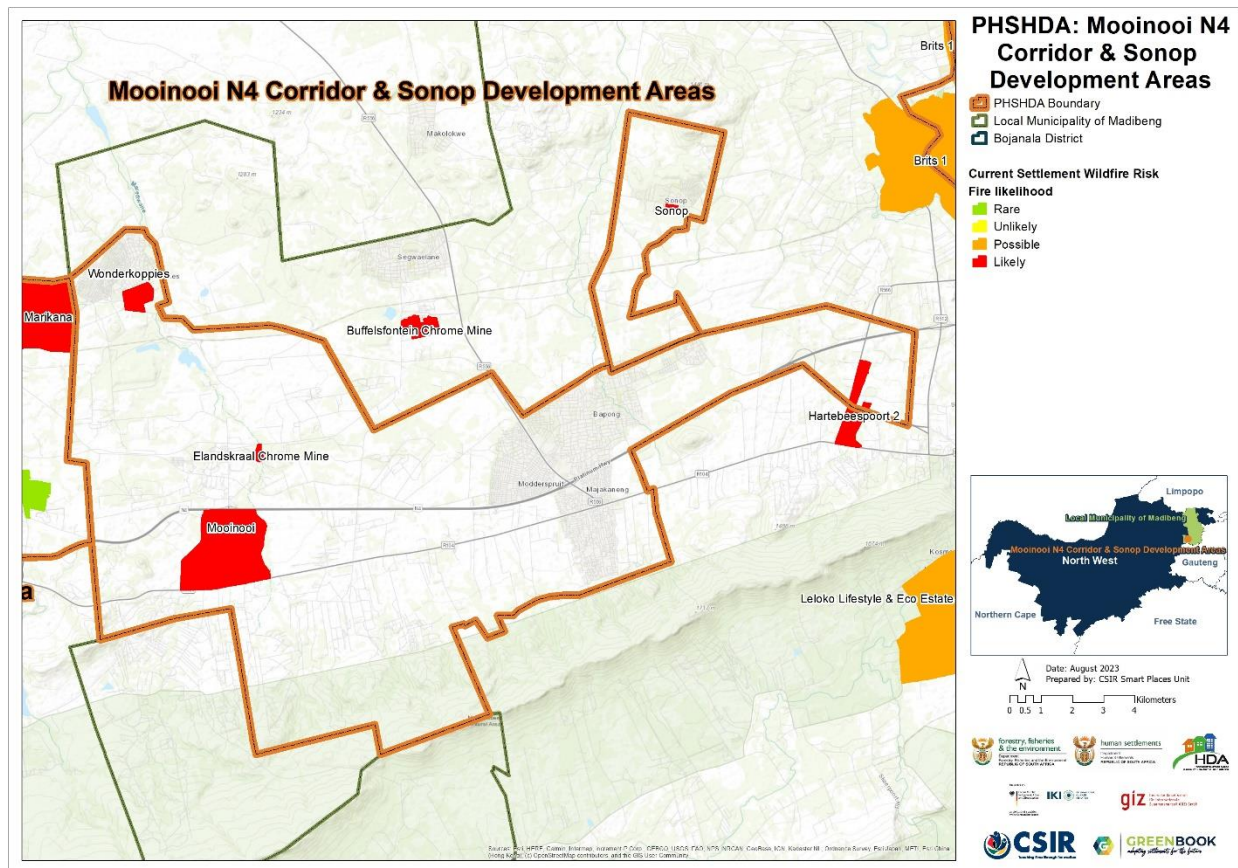
Figure 16: The likelihood of wildfires under current climatic conditions across settlements in the MCSDA PSHDA within Madibeng Local Municipality
